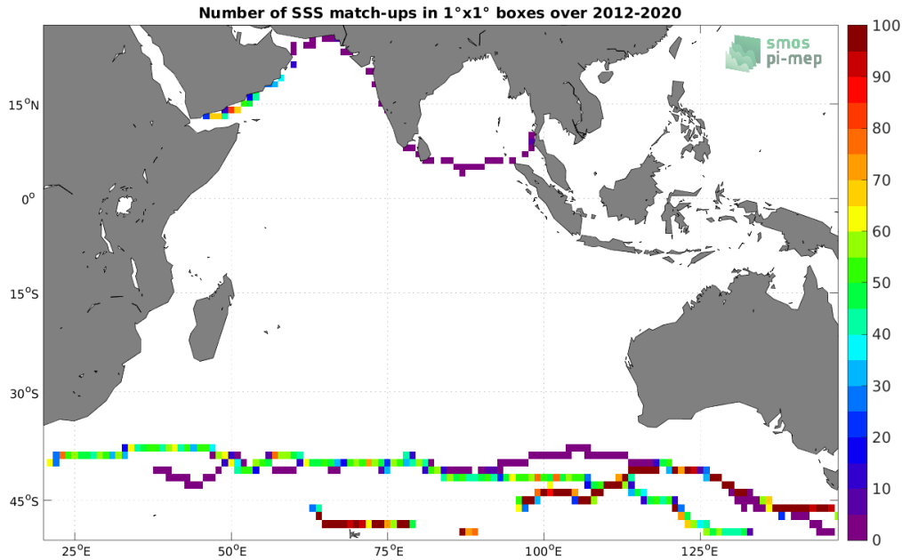
Figure 4: Number of SSS match-ups between TSG (GOSUD-Sailing-ship) SSS and the SMAP SSS L4 OI v1 - Monthly (IPRC) SSS product for the Indian Ocean Pi-MEP region over 1^\circ \times 1^\circ boxes and for the full satellite product period.
