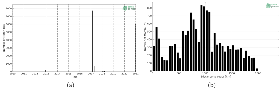
Figure 1: Number of match-ups between TSG (GOSUD-Sailing-ship) and SMAP SSS L4 OI v1 - Monthly (IPRC) SSS as a function of time (a) and as function of the distance to coast (b) over the Indian Ocean Pi-MEP region and for the full satellite product period.
