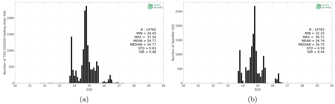
Figure 2: Histograms of SSS from TSG (GOSUD-Sailing-ship) (a) and SMAP SSS L4 OI v1 - Monthly (IPRC) (b) considering all match-up pairs per bins of 0.1 over the Indian Ocean Pi-MEP region and for the full satellite product period.
