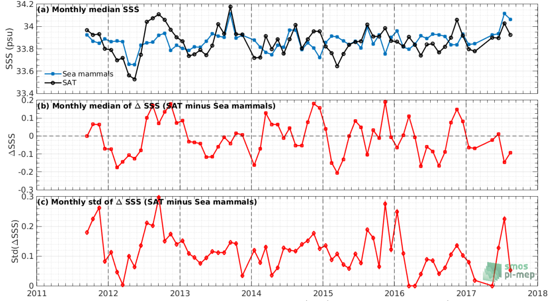
Figure 7: Time series of the monthly median SSS (top), median of \Delta\text{SSS} (Satellite - Marine mammals) and Std of \Delta\text{SSS} (Satellite - Marine mammals) over the Indian Ocean Pi-MEP region considering all match-ups collected by the Pi-MEP.
