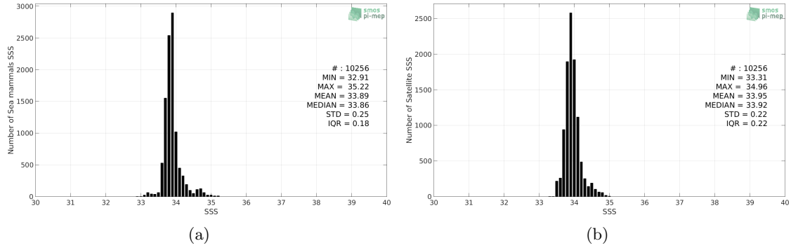
Figure 2: Histograms of SSS from Marine mammals (a) and SMAP SSS L4 OI v1 - Monthly (IPRC) (b) considering all match-up pairs per bins of 0.1 over the Indian Ocean Pi-MEP region and for the full satellite product period.
