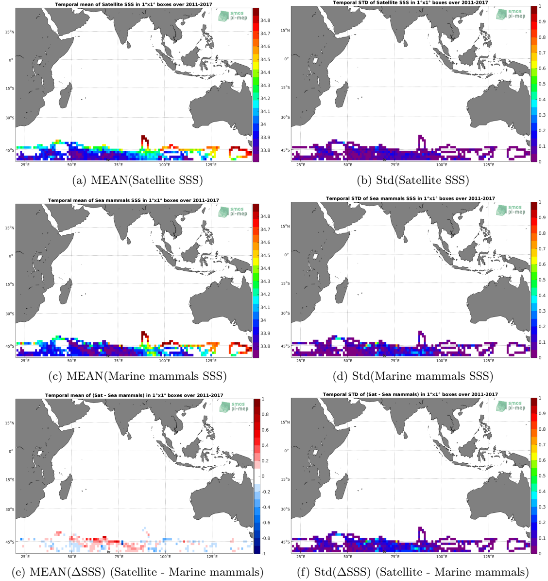
Figure 6: Temporal mean (left) and Std (right) of SSS from SMAP SSS L4 OI v1 - Monthly (IPRC) (top), Marine mammals (middle), and of \Delta SSS (Satellite - Marine mammals). Only match-up pairs are used to generate these maps.
