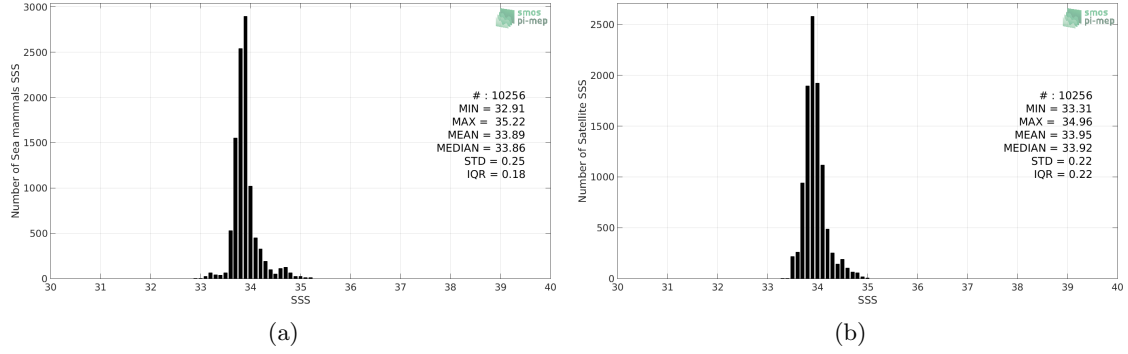
Figure 2: Histograms of SSS from Sea mammals (a) and SMAP SSS L4 OI v1 - Monthly (IPRC) (b) considering all match-up pairs per bins of 0.1 over the Indian Ocean Pi-MEP region and for the full satellite product period.
