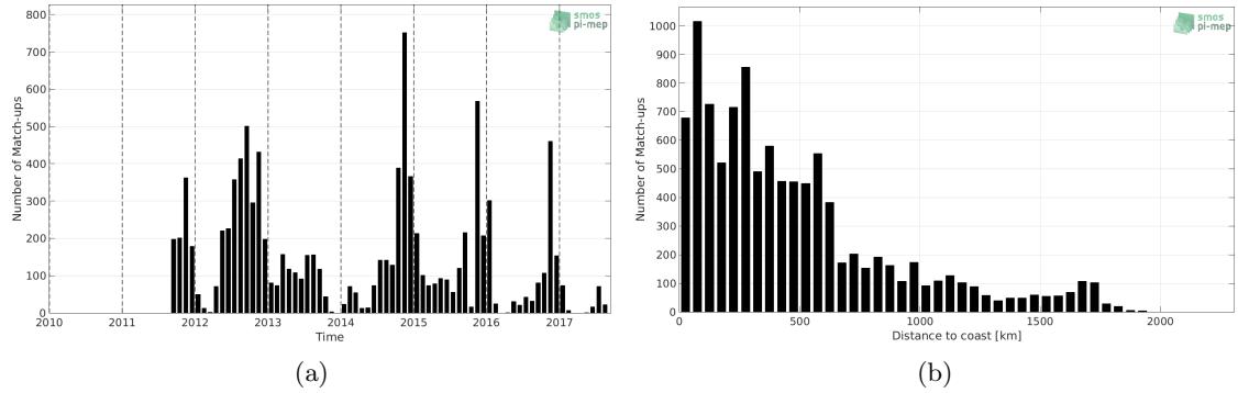
Figure 1: Number of match-ups between Sea mammals and SMAP SSS L4 OI v1 - Monthly (IPRC) SSS as a function of time (a) and as function of the distance to coast (b) over the Indian Ocean Pi-MEP region and for the full satellite product period.
