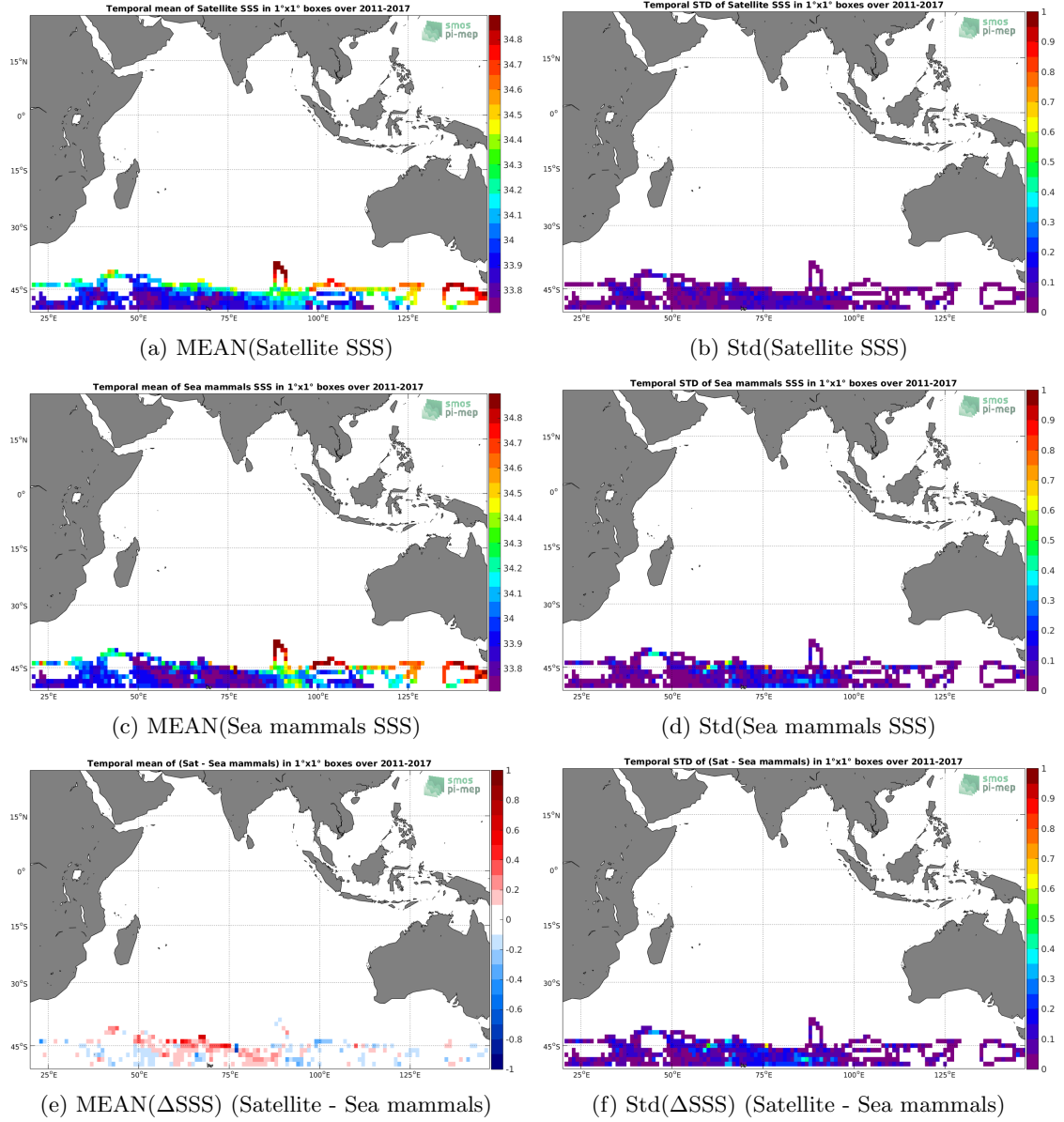
Figure 6: Temporal mean (left) and Std (right) of SSS from SMAP SSS L4 OI v1 - Monthly (IPRC) (top), Sea mammals (middle), and of \Delta SSS (Satellite - Sea mammals). Only match-up pairs are used to generate these maps.
