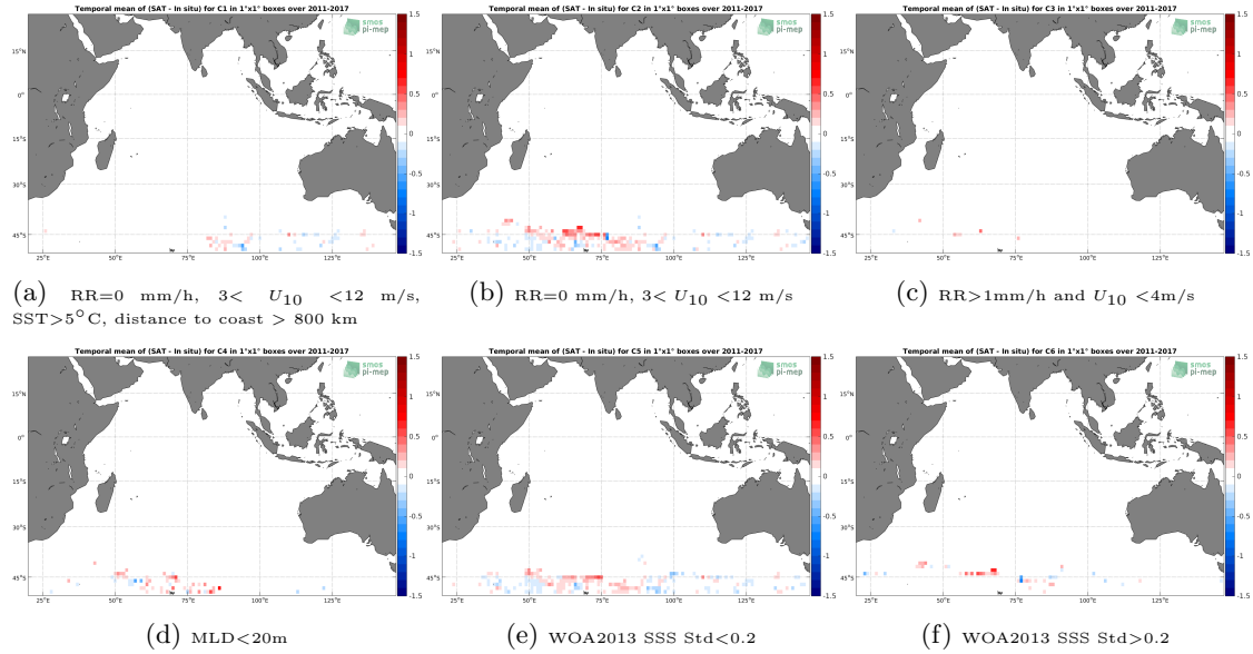
Figure 12: Temporal mean gridded over spatial boxes of size 1^{\circ}\times 1^{\circ} of \Delta\text{SSS} (SMAP SSS L4 OI v1 - Monthly (IPRC) - Sea mammals) for 6 different subdatasets corresponding to: \text{RR}=0 mm/h, 3 < U_{10} < 12 m/s, \text{SST} > 5^{\circ}\text{C} , distance to coast > 800 km (a), \text{RR}=0 mm/h, 3 < U_{10} < 12 m/s (b), \text{RR} > 1\text{mm/h} and U_{10} < 4\text{m/s} (c), \text{MLD} < 20\text{m} (d), \text{WOA2013 SSS Std} < 0.2 (e), \text{WOA2013 SSS Std} > 0.2 (f).
