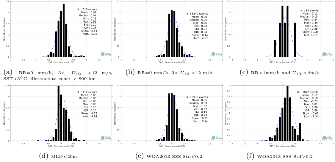
Figure 13: Normalized histogram of \Delta SSS (SMAP SSS L4 OI v1 - Monthly (IPRC) - Sea mammals) for 6 different subdatasets corresponding to: RR=0 mm/h, 3 < U_{10} < 12 m/s, SST>5°C, distance to coast > 800 km (a), RR=0 mm/h, 3 < U_{10} < 12 m/s (b), RR>1mm/h and U_{10} < 4 m/s (c), MLD<20m (d), WOA2013 SSS Std<0.2 (e), WOA2013 SSS Std>0.2 (f).
