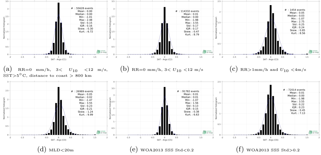
Figure 13: Normalized histogram of \Delta SSS (SMAP SSS L4 OI v1 - Monthly (IPRC) - Argo) for 6 different subdatasets corresponding to: RR=0 mm/h, 3 < U_{10} < 12 m/s, SST>5°C, distance to coast > 800 km (a), RR=0 mm/h, 3 < U_{10} < 12 m/s (b), RR>1mm/h and U_{10} < 4 m/s (c), MLD<20m (d), WOA2013 SSS Std<0.2 (e), WOA2013 SSS Std>0.2 (f).
