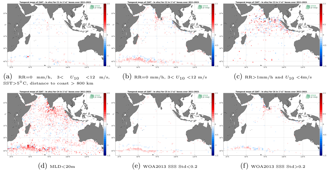
Figure 12: Temporal mean gridded over spatial boxes of size 1^\circ \times 1^\circ of \Delta SSS (SMAP SSS L4 OI v1 - Monthly (IPRC) - Argo) for 6 different subdatasets corresponding to: RR=0 mm/h, 3 < U_{10} < 12 m/s, SST > 5^\circ C , distance to coast > 800 km (a), RR=0 mm/h, 3 < U_{10} < 12 m/s (b), RR > 1 mm/h and U_{10} < 4 m/s (c), MLD < 20 m (d), WOA2013 SSS Std < 0.2 (e), WOA2013 SSS Std > 0.2 (f).
