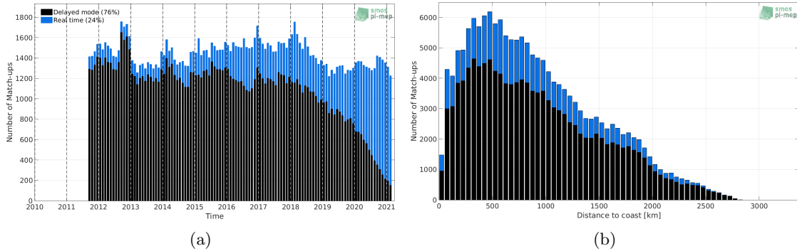
Figure 1: Number of match-ups between Argo and SMAP SSS L4 OI v1 - Monthly (IPRC) SSS as a function of time (a) and as function of the distance to coast (b) over the Indian Ocean Pi-MEP region and for the full satellite product period.
