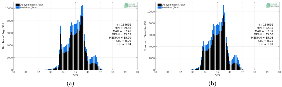
Figure 2: Histograms of SSS from Argo (a) and SMAP SSS L4 OI v1 - Monthly (IPRC) (b) considering all match-up pairs per bins of 0.1 over the Indian Ocean Pi-MEP region and for the full satellite product period.
