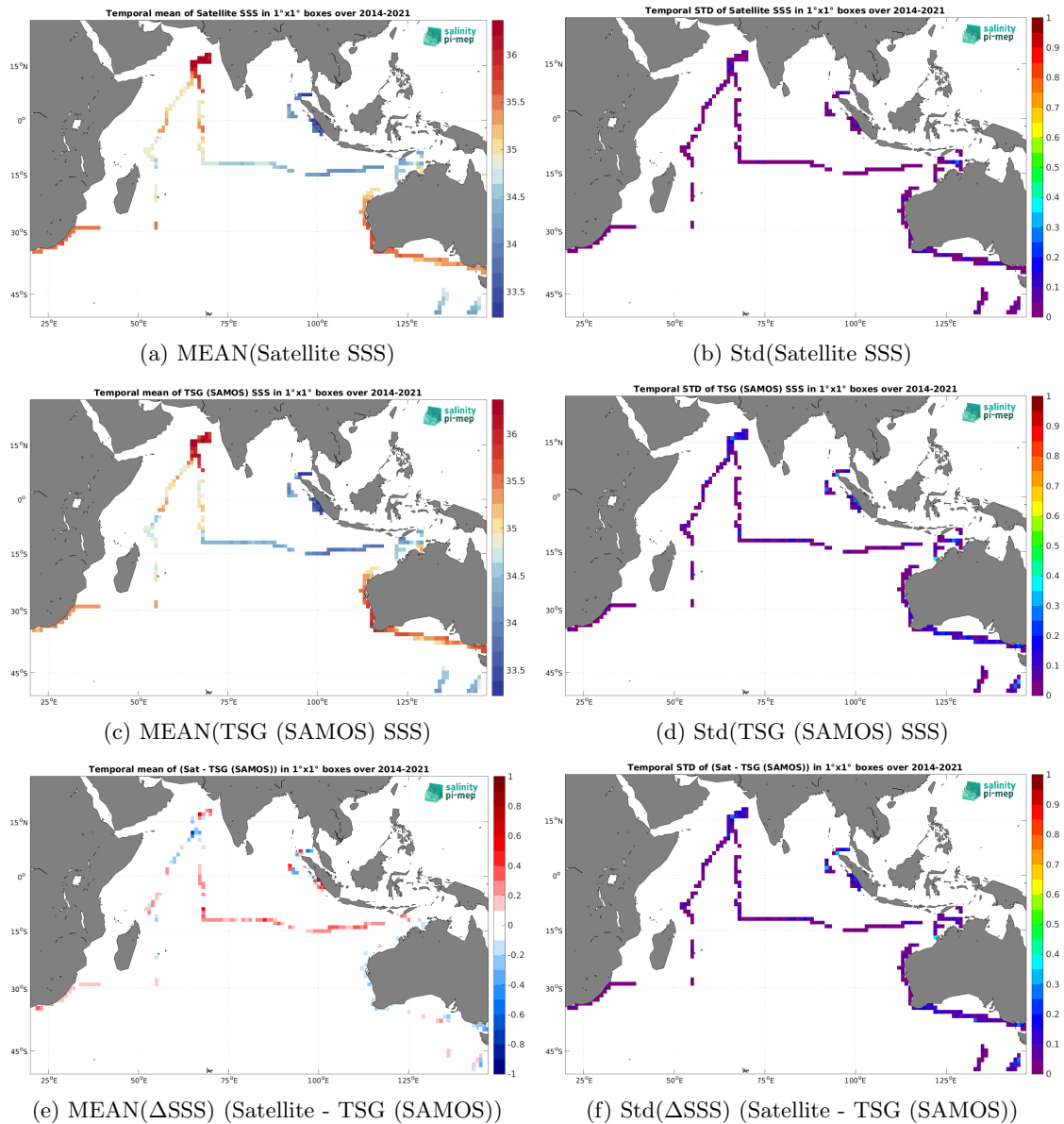
Figure 7: Temporal mean (left) and Std (right) of SSS from SMAP SSS L4 OI v3 - Monthly (ESR) (top), TSG (SAMOS) (middle), and of \Delta SSS (Satellite - TSG (SAMOS)). Only match-up pairs are used to generate these maps.
