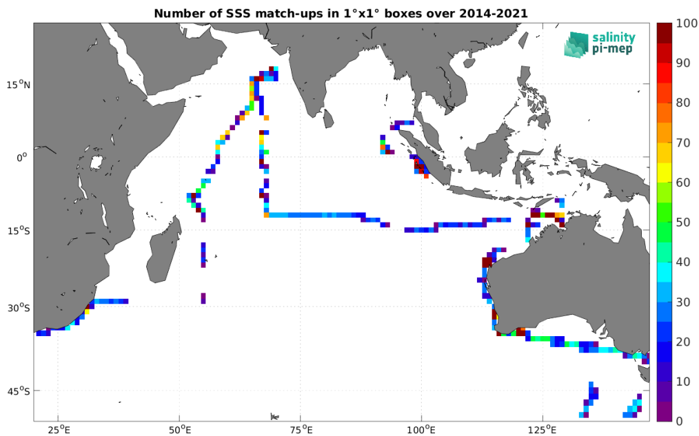
Figure 5: Number of SSS match-ups between TSG (SAMOS) SSS and the SMAP SSS L4 OI v3 - Monthly (ESR) SSS product for the Indian Ocean Pi-MEP region over 1^\circ \times 1^\circ boxes and for the full satellite product period.
