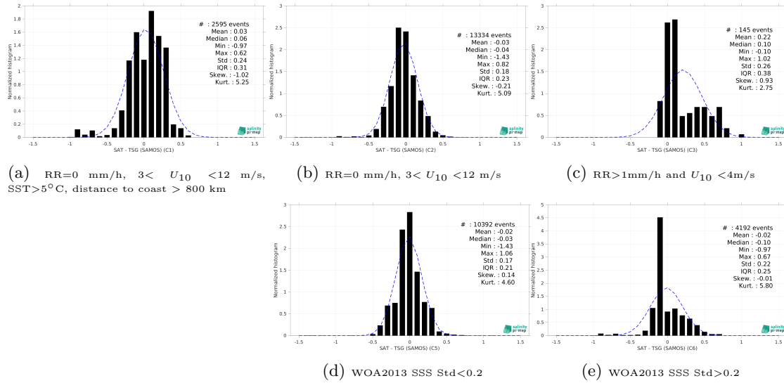
Figure 15: Normalized histogram of \Delta\text{SSS} (SMAP SSS L4 OI v3 - Monthly (ESR) - TSG (SAMOS)) for 5 different subdatasets corresponding to: RR=0 mm/h, 3 < U_{10} < 12 m/s, SST>5°C, distance to coast > 800 km (a), RR=0 mm/h, 3 < U_{10} < 12 m/s (b), RR>1mm/h and U_{10} < 4 m/s (c), WOA2013 SSS Std<0.2 (d), WOA2013 SSS Std>0.2 (e).
