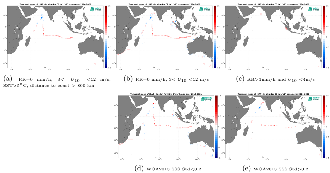
Figure 14: Temporal mean gridded over spatial boxes of size 1^\circ \times 1^\circ of \Delta SSS (SMAP SSS L4 OI v3 - Monthly (ESR) - TSG (SAMOS)) for 5 different subdatasets corresponding to:RR=0 mm/h, 3 < U_{10} < 12 m/s, SST >5^\circ C, distance to coast > 800 km (a), RR=0 mm/h, 3 < U_{10} < 12 m/s (b), RR >1 mm/h and U_{10} < 4 m/s (c), WOA2013 SSS Std <0.2 (d), WOA2013 SSS Std >0.2 (e).
