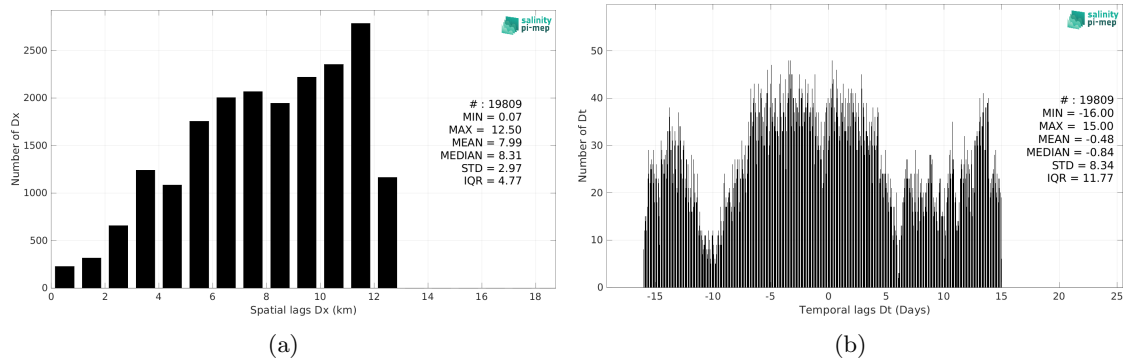
Figure 6: Histograms of the spatial (a) and temporal (b) lags between the location/time of the TSG (SAMOS) measurement and the date of the corresponding SMAP SSS L4 OI v3 - Monthly (ESR) SSS pixel.
