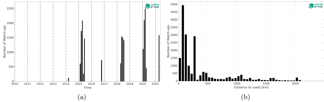
Figure 2: Number of match-ups between TSG (SAMOS) and SMAP SSS L4 OI v3 - Monthly (ESR) SSS as a function of time (a) and as function of the distance to coast (b) over the Indian Ocean Pi-MEP region and for the full satellite product period.
