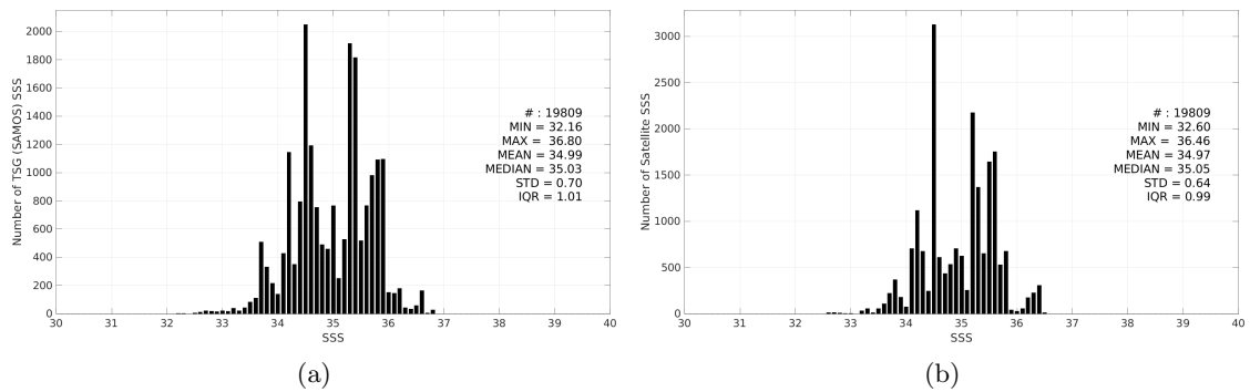
Figure 3: Histograms of SSS from TSG (SAMOS) (a) and SMAP SSS L4 OI v3 - Monthly (ESR) (b) considering all match-up pairs per bins of 0.1 over the Indian Ocean Pi-MEP region and for the full satellite product period.
