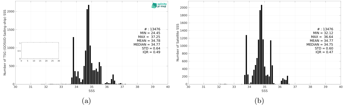
Figure 3: Histograms of SSS from TSG (GOSUD-Sailing-ship) (a) and SMAP SSS L4 OI v3 - Monthly (ESR) (b) considering all match-up pairs per bins of 0.1 over the Indian Ocean Pi-MEP region and for the full satellite product period.
