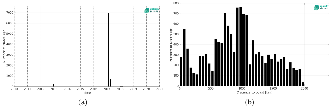
Figure 2: Number of match-ups between TSG (GOSUD-Sailing-ship) and SMAP SSS L4 OI v3 - Monthly (ESR) SSS as a function of time (a) and as function of the distance to coast (b) over the Indian Ocean Pi-MEP region and for the full satellite product period.
