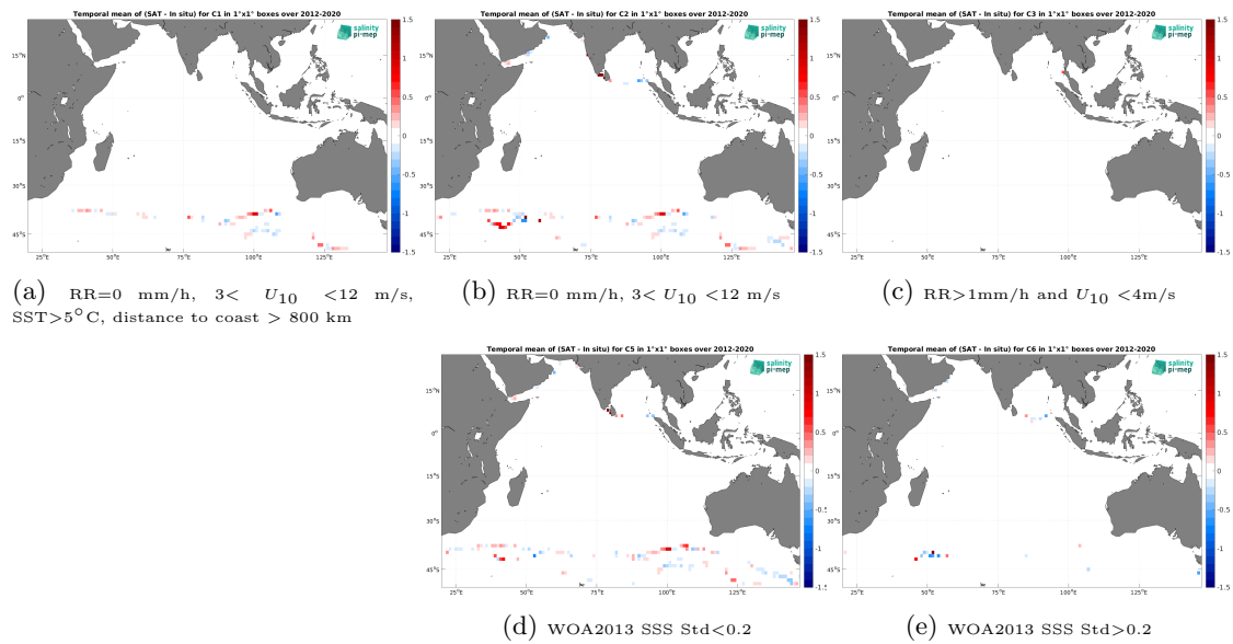
Figure 14: Temporal mean gridded over spatial boxes of size 1^\circ \times 1^\circ of \Delta SSS (SMAP SSS L4 OI v3 - Monthly (ESR) - TSG (GOSUD-Sailing-ship)) for 5 different subdatasets corresponding to:RR=0 mm/h, 3 < U_{10} < 12 m/s, SST > 5^\circ\text{C} , distance to coast > 800 km (a), RR=0 mm/h, 3 < U_{10} < 12 m/s (b), RR > 1 mm/h and U_{10} < 4 m/s (c), WOA2013 SSS Std < 0.2 (d), WOA2013 SSS Std > 0.2 (e).
