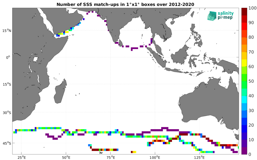
Figure 5: Number of SSS match-ups between TSG (GOSUD-Sailing-ship) SSS and the SMAP SSS L4 OI v3 - Monthly (ESR) SSS product for the Indian Ocean Pi-MEP region over 1^\circ \times 1^\circ boxes and for the full satellite product period.
