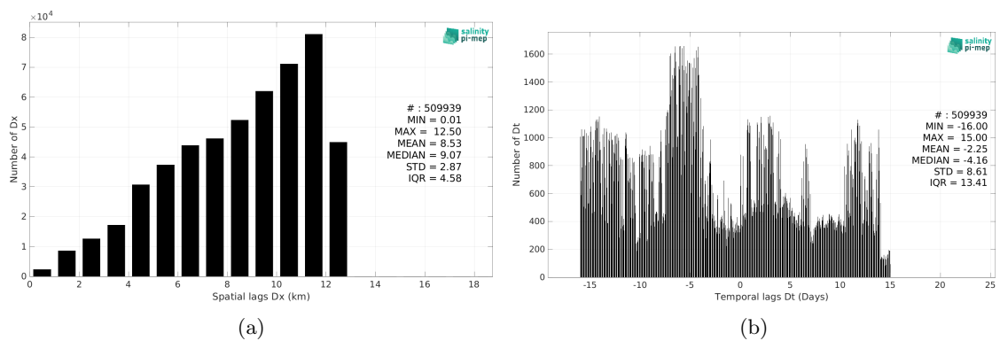
Figure 6: Histograms of the spatial (a) and temporal (b) lags between the location/time of the TSG (GOSUD-Research-vessel) measurement and the date of the corresponding SMAP SSS L4 OI v3 - Monthly (ESR) SSS pixel.
