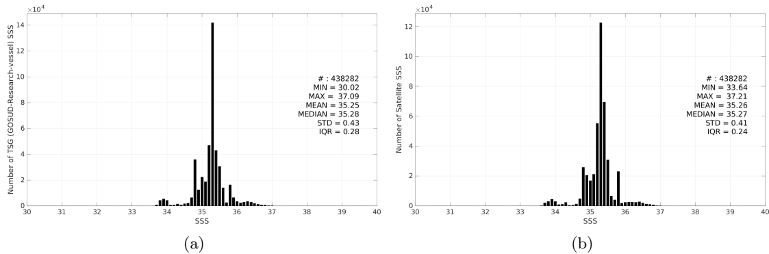
Figure 3: Histograms of SSS from TSG (GOSUD-Research-vessel) (a) and SMAP SSS L4 OI v3 - Monthly (ESR) (b) considering all match-up pairs per bins of 0.1 over the Indian Ocean Pi-MEP region and for the full satellite product period.
