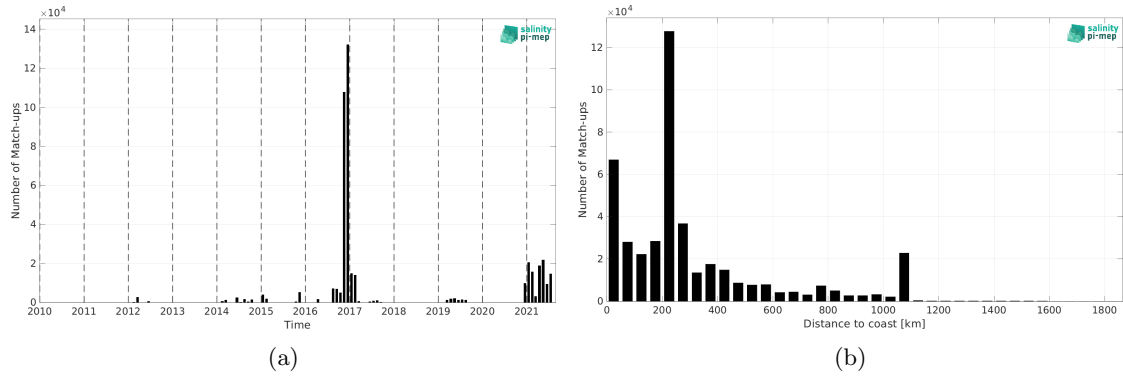
Figure 2: Number of match-ups between TSG (GOSUD-Research-vessel) and SMAP SSS L4 OI v3 - Monthly (ESR) SSS as a function of time (a) and as function of the distance to coast (b) over the Indian Ocean Pi-MEP region and for the full satellite product period.
