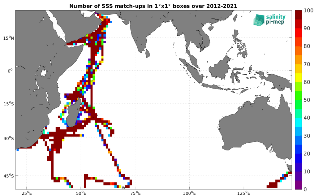
Figure 5: Number of SSS match-ups between TSG (GOSUD-Research-vessel) SSS and the SMAP SSS L4 OI v3 - Monthly (ESR) SSS product for the Indian Ocean Pi-MEP region over 1^\circ \times 1^\circ boxes and for the full satellite product period.
