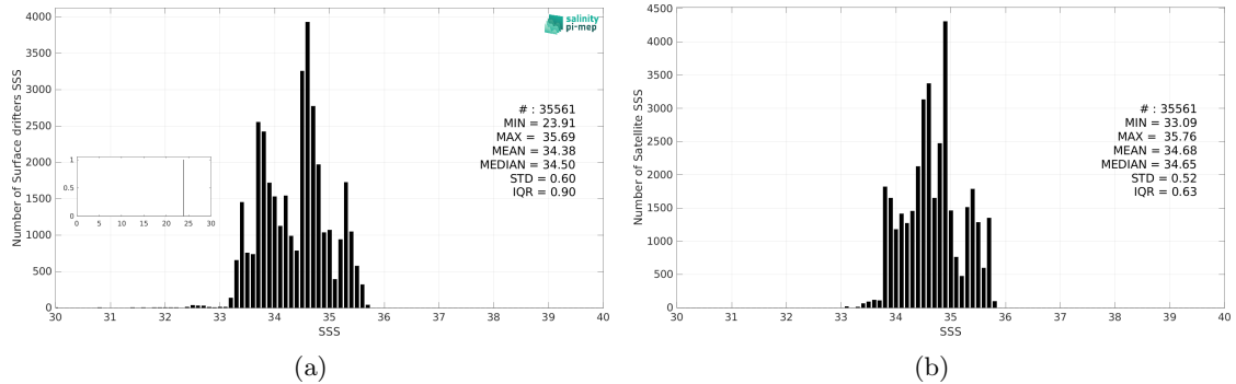
Figure 3: Histograms of SSS from Surface drifters (a) and SMAP SSS L4 OI v3 - Monthly (ESR) (b) considering all match-up pairs per bins of 0.1 over the Indian Ocean Pi-MEP region and for the full satellite product period.
