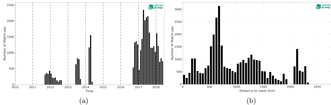
Figure 2: Number of match-ups between Surface drifters and SMAP SSS L4 OI v3 - Monthly (ESR) SSS as a function of time (a) and as function of the distance to coast (b) over the Indian Ocean Pi-MEP region and for the full satellite product period.
