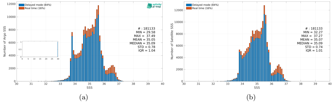
Figure 3: Histograms of SSS from Argo (a) and SMAP SSS L4 OI v3 - Monthly (ESR) (b) considering all match-up pairs per bins of 0.1 over the Indian Ocean Pi-MEP region and for the full satellite product period.
