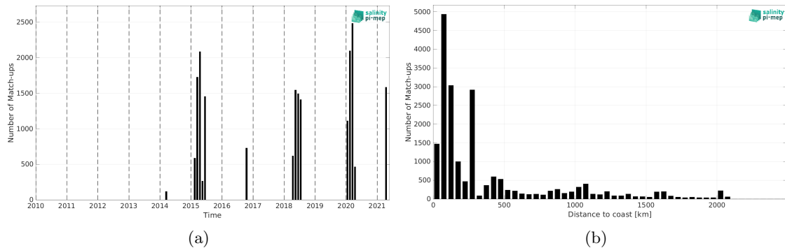
Figure 2: Number of match-ups between TSG (SAMOS) and SMAP SSS L4 OI v3 - Daily (ESR) SSS as a function of time (a) and as function of the distance to coast (b) over the Indian Ocean Pi-MEP region and for the full satellite product period.
