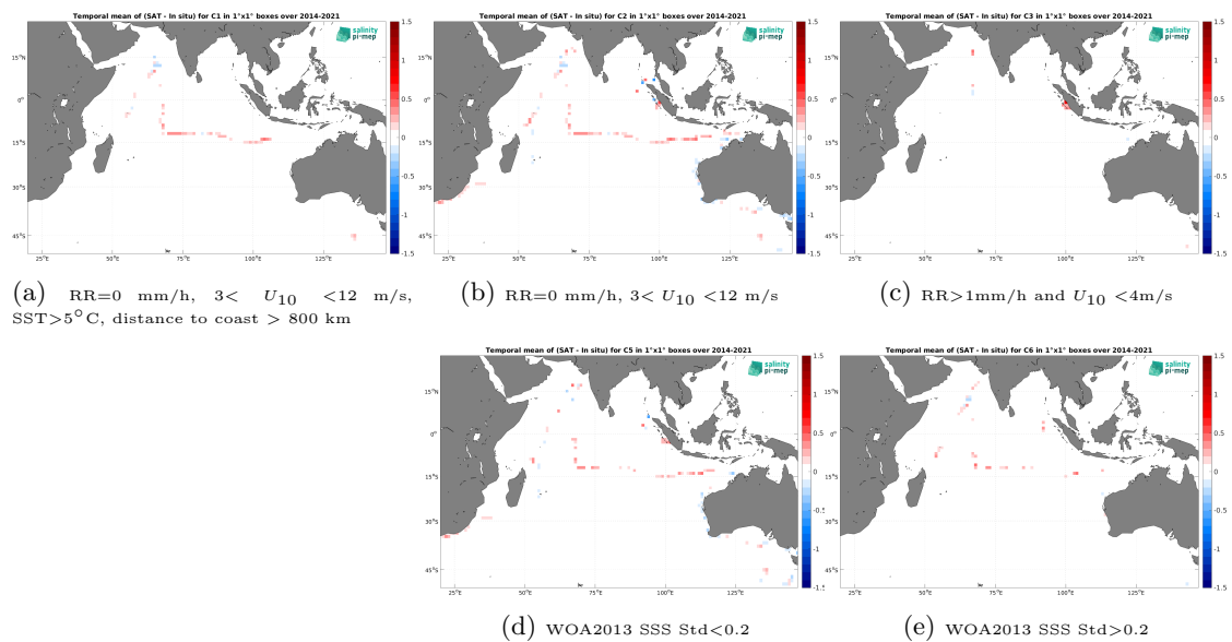
Figure 14: Temporal mean gridded over spatial boxes of size 1^\circ \times 1^\circ of \Delta SSS (SMAP SSS L4 OI v3 - Daily (ESR) - TSG (SAMOS)) for 5 different subdatasets corresponding to:RR=0 mm/h, 3 < U_{10} < 12 m/s, SST > 5^\circ\text{C} , distance to coast > 800 km (a), RR=0 mm/h, 3 < U_{10} < 12 m/s (b), RR > 1 mm/h and U_{10} < 4 m/s (c), WOA2013 SSS Std < 0.2 (d), WOA2013 SSS Std > 0.2 (e).
