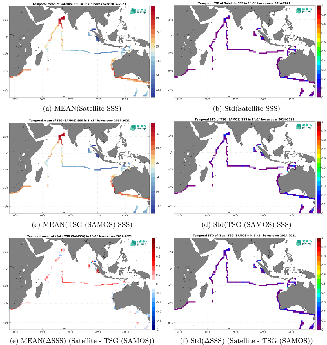
Figure 7: Temporal mean (left) and Std (right) of SSS from SMAP SSS L4 OI v3 - Daily (ESR) (top), TSG (SAMOS) (middle), and of \Delta SSS (Satellite - TSG (SAMOS)). Only match-up pairs are used to generate these maps.
