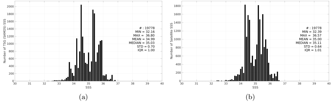
Figure 3: Histograms of SSS from TSG (SAMOS) (a) and SMAP SSS L4 OI v3 - Daily (ESR) (b) considering all match-up pairs per bins of 0.1 over the Indian Ocean Pi-MEP region and for the full satellite product period.
