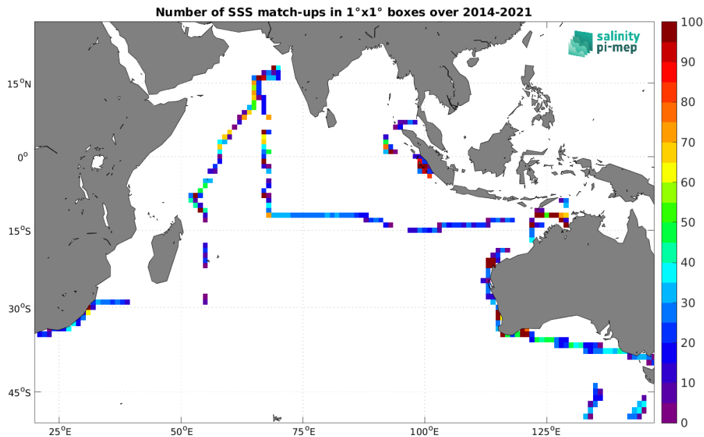
Figure 5: Number of SSS match-ups between TSG (SAMOS) SSS and the SMAP SSS L4 OI v3 - Daily (ESR) SSS product for the Indian Ocean Pi-MEP region over 1^\circ \times 1^\circ boxes and for the full satellite product period.
