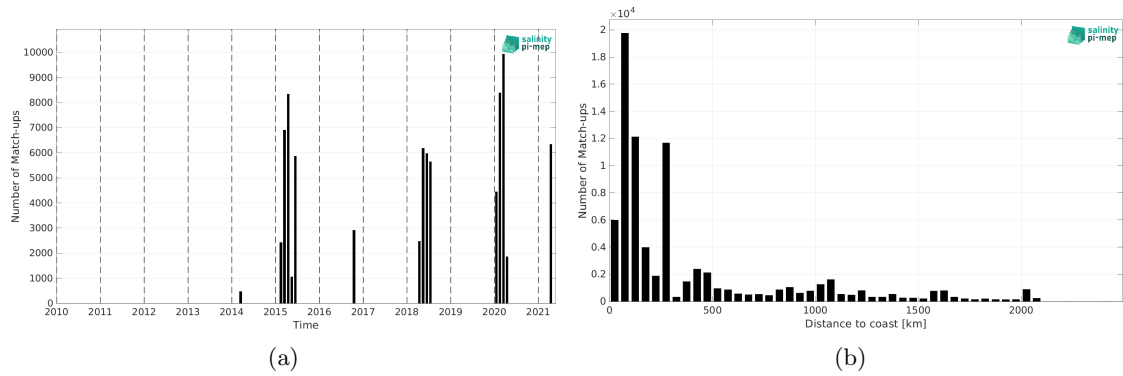
Figure 2: Number of match-ups between TSG (SAMOS) and SMAP SSS L4 OI v3 - Daily (ESR) SSS as a function of time (a) and as function of the distance to coast (b) over the Indian Ocean Pi-MEP region and for the full satellite product period.
