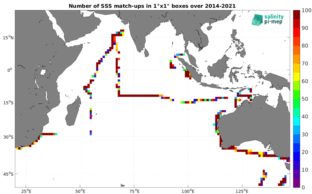
Figure 5: Number of SSS match-ups between TSG (SAMOS) SSS and the SMAP SSS L4 OI v3 - Daily (ESR) SSS product for the Indian Ocean Pi-MEP region over 1^\circ \times 1^\circ boxes and for the full satellite product period.
