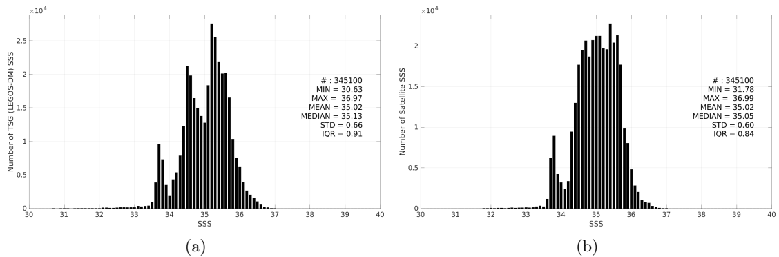
Figure 3: Histograms of SSS from TSG (LEGOS-DM) (a) and SMAP SSS L4 OI v3 - Daily (ESR) (b) considering all match-up pairs per bins of 0.1 over the Indian Ocean Pi-MEP region and for the full satellite product period.
