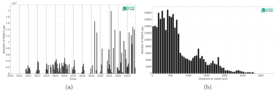
Figure 2: Number of match-ups between TSG (LEGOS-DM) and SMAP SSS L4 OI v3 - Daily (ESR) SSS as a function of time (a) and as function of the distance to coast (b) over the Indian Ocean Pi-MEP region and for the full satellite product period.
