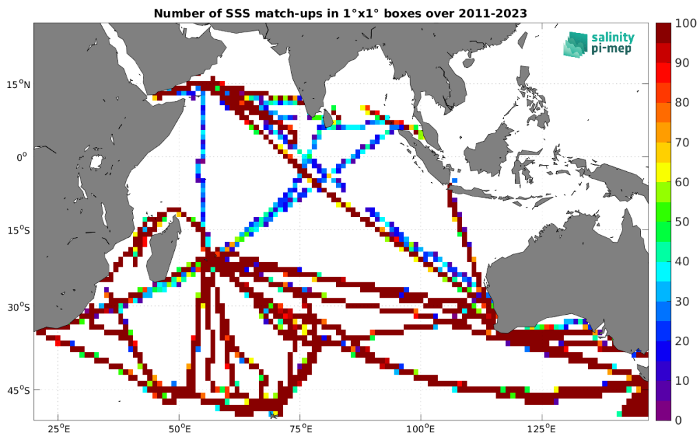
Figure 5: Number of SSS match-ups between TSG (LEGOS-DM) SSS and the SMAP SSS L4 OI v3 - Daily (ESR) SSS product for the Indian Ocean Pi-MEP region over 1^\circ \times 1^\circ boxes and for the full satellite product period.
