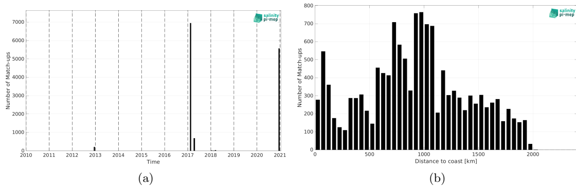
Figure 2: Number of match-ups between TSG (GOSUD-Sailing-ship) and SMAP SSS L4 OI v3 - Daily (ESR) SSS as a function of time (a) and as function of the distance to coast (b) over the Indian Ocean Pi-MEP region and for the full satellite product period.
