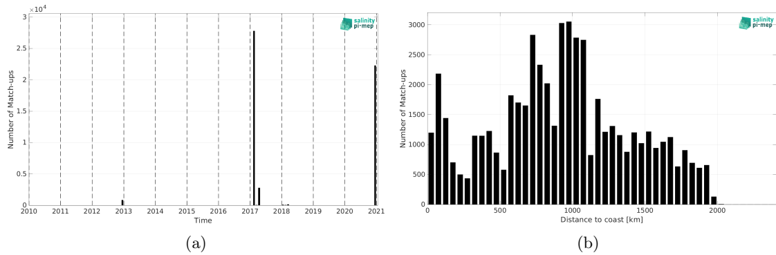
Figure 2: Number of match-ups between TSG (GOSUD-Sailing-ship) and SMAP SSS L4 OI v3 - Daily (ESR) SSS as a function of time (a) and as function of the distance to coast (b) over the Indian Ocean Pi-MEP region and for the full satellite product period.
