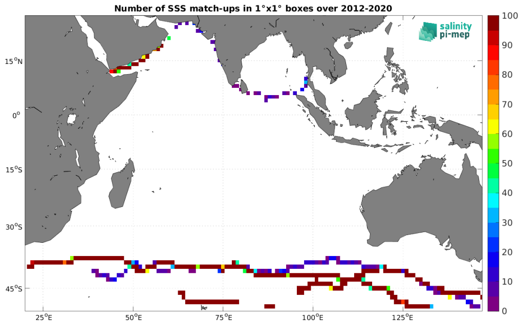
Figure 5: Number of SSS match-ups between TSG (GOSUD-Sailing-ship) SSS and the SMAP SSS L4 OI v3 - Daily (ESR) SSS product for the Indian Ocean Pi-MEP region over 1^\circ \times 1^\circ boxes and for the full satellite product period.
