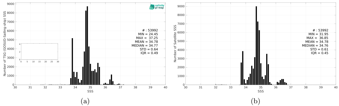
Figure 3: Histograms of SSS from TSG (GOSUD-Sailing-ship) (a) and SMAP SSS L4 OI v3 - Daily (ESR) (b) considering all match-up pairs per bins of 0.1 over the Indian Ocean Pi-MEP region and for the full satellite product period.
