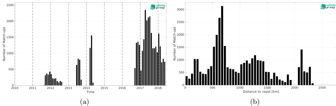
Figure 2: Number of match-ups between Surface drifters and SMAP SSS L4 OI v3 - Daily (ESR) SSS as a function of time (a) and as function of the distance to coast (b) over the Indian Ocean Pi-MEP region and for the full satellite product period.
