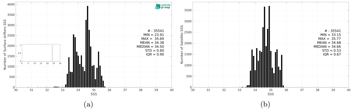
Figure 3: Histograms of SSS from Surface drifters (a) and SMAP SSS L4 OI v3 - Daily (ESR) (b) considering all match-up pairs per bins of 0.1 over the Indian Ocean Pi-MEP region and for the full satellite product period.
