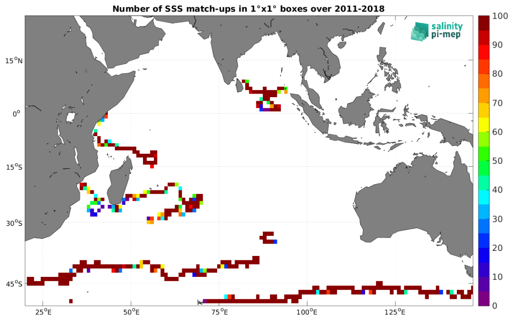
Figure 4: Number of SSS match-ups between Surface drifters SSS and the SMAP SSS L4 OI v3 - Daily (ESR) SSS product for the Indian Ocean Pi-MEP region over 1^\circ \times 1^\circ boxes and for the full satellite product period.
