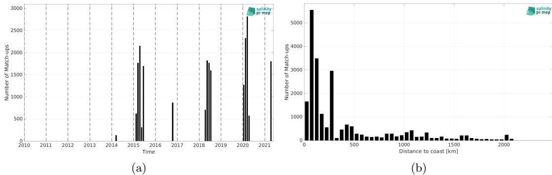
Figure 1: Number of match-ups between TSG (SAMOS) and SMAP SSS L4 OI v2 - 7 Days (ESR) SSS as a function of time (a) and as function of the distance to coast (b) over the Indian Ocean Pi-MEP region and for the full satellite product period.
