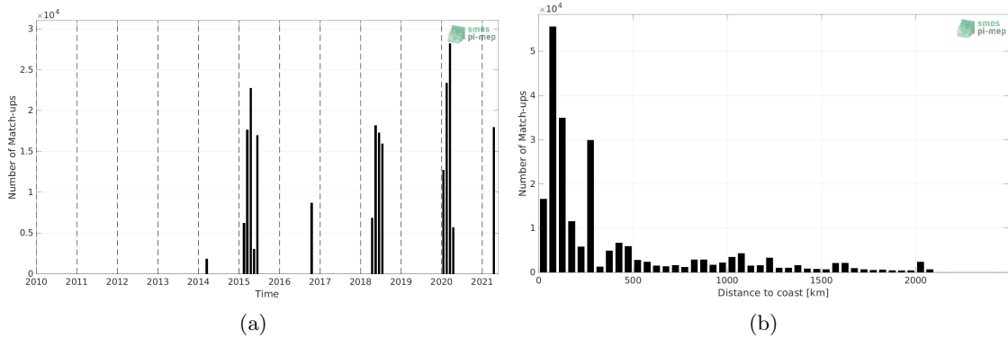
Figure 1: Number of match-ups between TSG (SAMOS) and SMAP SSS L4 OI v2 - 7 Days (ESR) SSS as a function of time (a) and as function of the distance to coast (b) over the Indian Ocean Pi-MEP region and for the full satellite product period.
