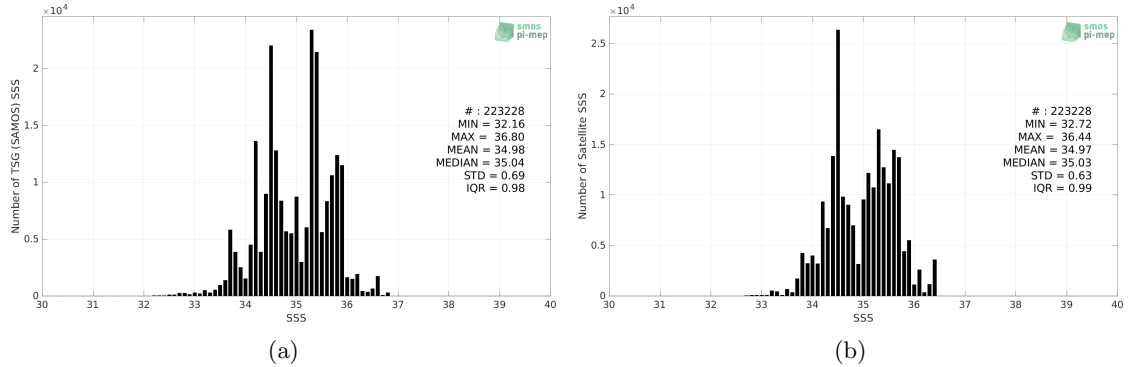
Figure 2: Histograms of SSS from TSG (SAMOS) (a) and SMAP SSS L4 OI v2 - 7 Days (ESR) (b) considering all match-up pairs per bins of 0.1 over the Indian Ocean Pi-MEP region and for the full satellite product period.
