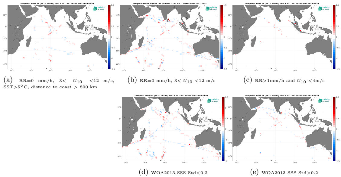
Figure 12: Temporal mean gridded over spatial boxes of size 1^\circ \times 1^\circ of \Delta SSS (SMAP SSS L4 OI v2 - 7 Days (ESR) - TSG (LEGOS-DM)) for 5 different subdatasets corresponding to:RR=0 mm/h, 3 < U_{10} < 12 m/s, SST >5^\circ\text{C} , distance to coast > 800 km (a), RR=0 mm/h, 3 < U_{10} < 12 m/s (b), RR >1 mm/h and U_{10} < 4 m/s (c), WOA2013 SSS Std <0.2 (d), WOA2013 SSS Std >0.2 (e).
