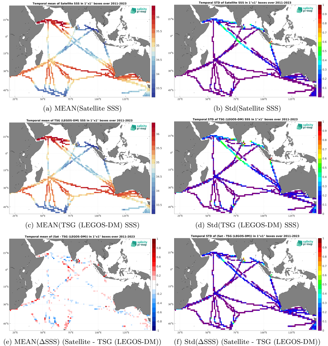
Figure 6: Temporal mean (left) and Std (right) of SSS from SMAP SSS L4 OI v2 - 7 Days (ESR) (top), TSG (LEGOS-DM) (middle), and of \Delta SSS (Satellite - TSG (LEGOS-DM)). Only match-up pairs are used to generate these maps.
