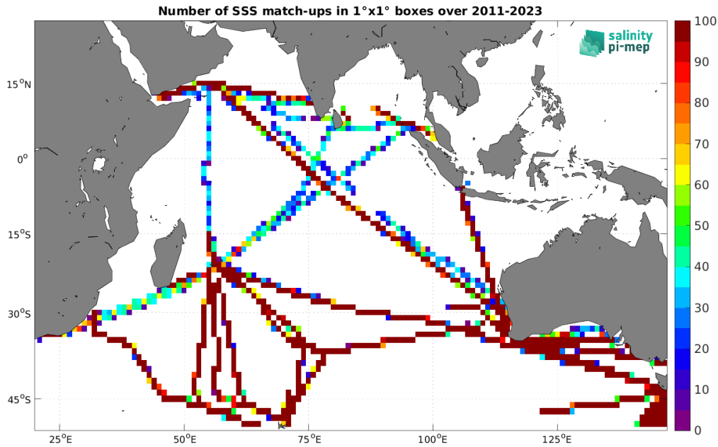
Figure 4: Number of SSS match-ups between TSG (LEGOS-DM) SSS and the SMAP SSS L4 OI v2 - 7 Days (ESR) SSS product for the Indian Ocean Pi-MEP region over 1^\circ \times 1^\circ boxes and for the full satellite product period.
