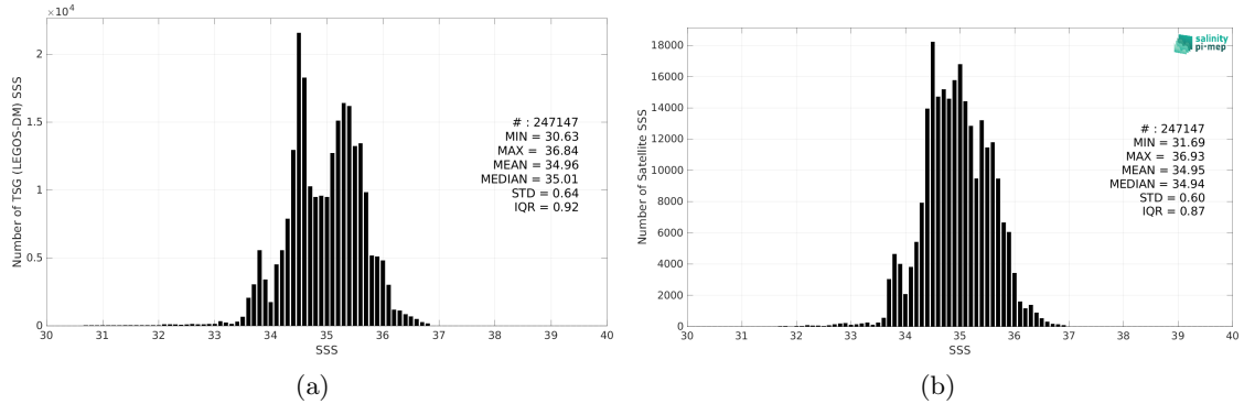
Figure 2: Histograms of SSS from TSG (LEGOS-DM) (a) and SMAP SSS L4 OI v2 - 7 Days (ESR) (b) considering all match-up pairs per bins of 0.1 over the Indian Ocean Pi-MEP region and for the full satellite product period.
