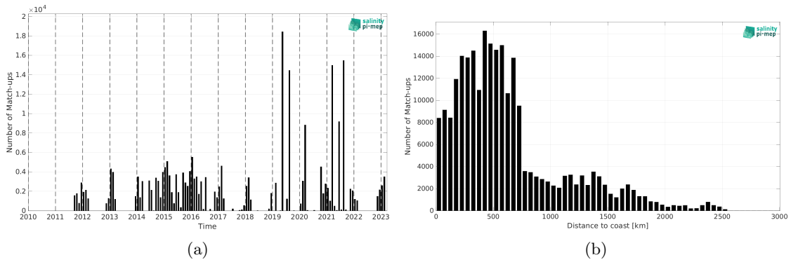
Figure 1: Number of match-ups between TSG (LEGOS-DM) and SMAP SSS L4 OI v2 - 7 Days (ESR) SSS as a function of time (a) and as function of the distance to coast (b) over the Indian Ocean Pi-MEP region and for the full satellite product period.
