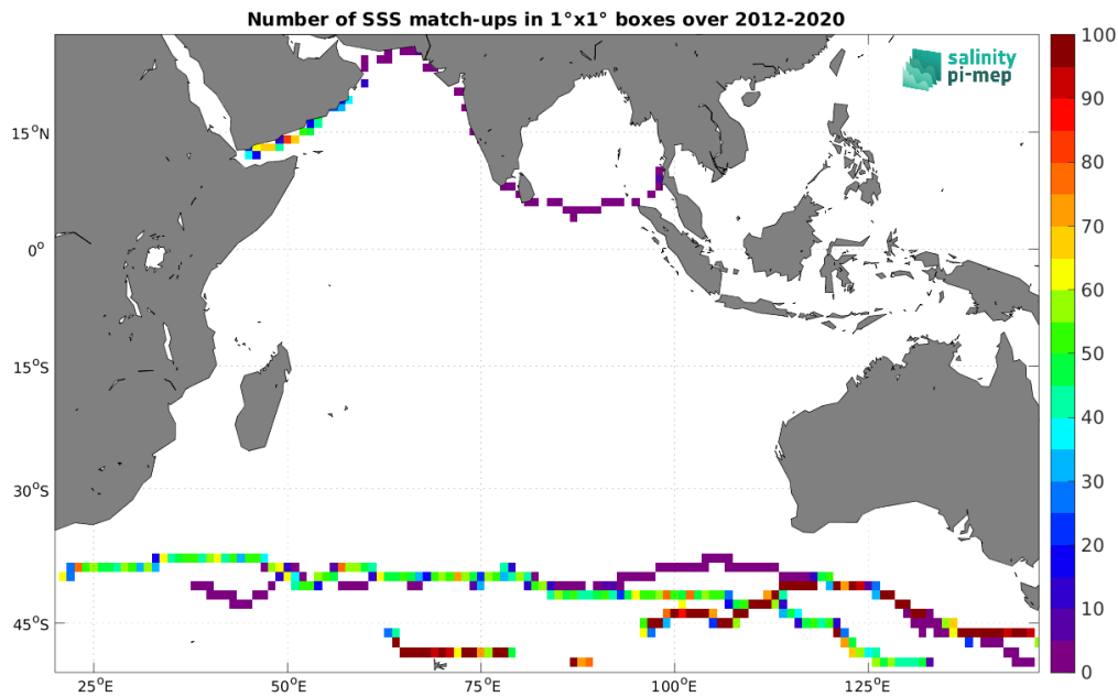
Figure 4: Number of SSS match-ups between TSG (GOSUD-Sailing-ship) SSS and the SMAP SSS L4 OI v2 - 7 Days (ESR) SSS product for the Indian Ocean Pi-MEP region over 1^\circ \times 1^\circ boxes and for the full satellite product period.
