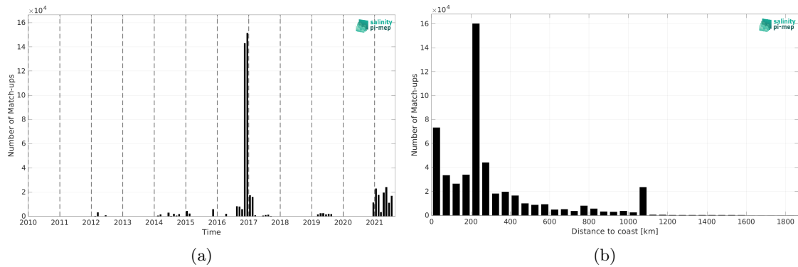
Figure 1: Number of match-ups between TSG (GOSUD-Research-vessel) and SMAP SSS L4 OI v2 - 7 Days (ESR) SSS as a function of time (a) and as function of the distance to coast (b) over the Indian Ocean Pi-MEP region and for the full satellite product period.
