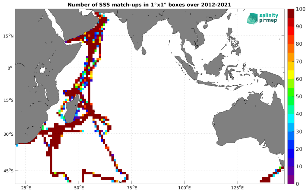
Figure 4: Number of SSS match-ups between TSG (GOSUD-Research-vessel) SSS and the SMAP SSS L4 OI v2 - 7 Days (ESR) SSS product for the Indian Ocean Pi-MEP region over 1^\circ \times 1^\circ boxes and for the full satellite product period.
