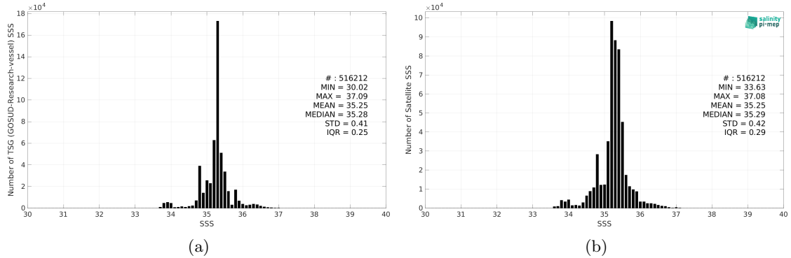
Figure 2: Histograms of SSS from TSG (GOSUD-Research-vessel) (a) and SMAP SSS L4 OI v2 - 7 Days (ESR) (b) considering all match-up pairs per bins of 0.1 over the Indian Ocean Pi-MEP region and for the full satellite product period.
