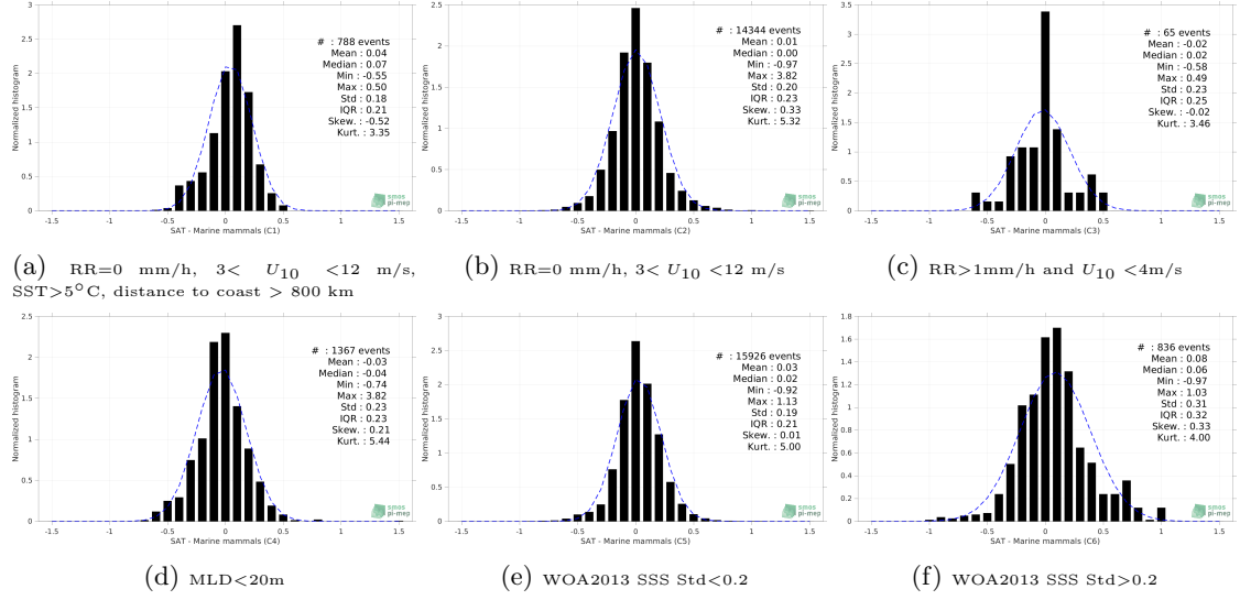
Figure 13: Normalized histogram of \Delta SSS (SMAP SSS L4 OI v2 - 7 Days (ESR) - Marine mammals) for 6 different subdatasets corresponding to: RR=0 mm/h, 3 < U_{10} < 12 m/s, SST>5°C, distance to coast > 800 km (a), RR=0 mm/h, 3 < U_{10} < 12 m/s (b), RR>1mm/h and U_{10} < 4 m/s (c), MLD<20m (d), WOA2013 SSS Std<0.2 (e), WOA2013 SSS Std>0.2 (f).
