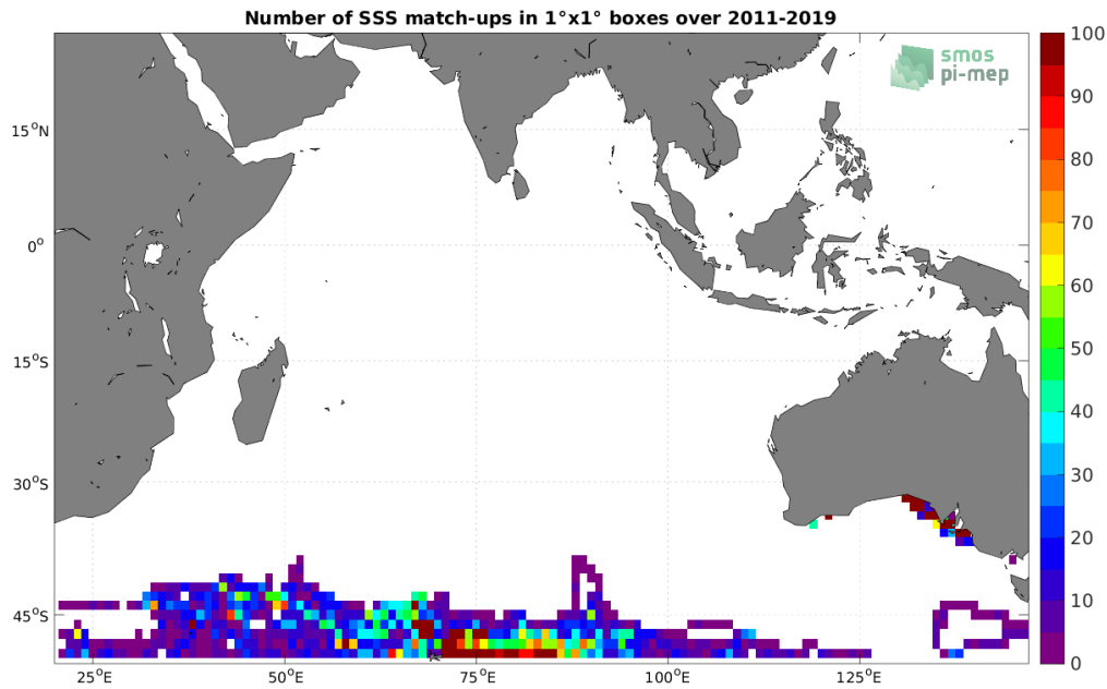
Figure 4: Number of SSS match-ups between Marine mammals SSS and the SMAP SSS L4 OI v2 - 7 Days (ESR) SSS product for the Indian Ocean Pi-MEP region over 1^\circ \times 1^\circ boxes and for the full satellite product period.
