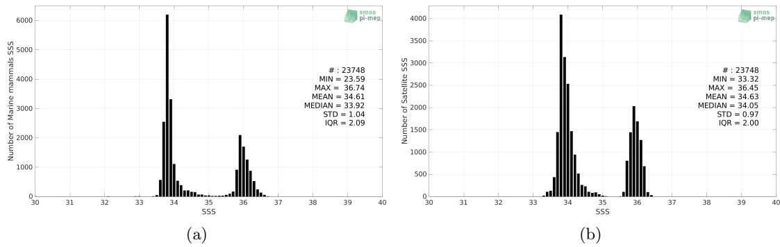
Figure 2: Histograms of SSS from Marine mammals (a) and SMAP SSS L4 OI v2 - 7 Days (ESR) (b) considering all match-up pairs per bins of 0.1 over the Indian Ocean Pi-MEP region and for the full satellite product period.
