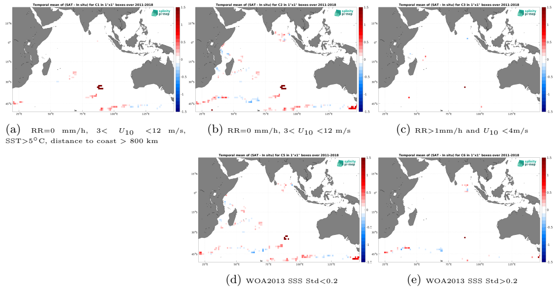
Figure 11: Temporal mean gridded over spatial boxes of size 1^\circ \times 1^\circ of \Delta SSS (SMAP SSS L4 OI v2 - 7 Days (ESR) - Surface drifters) for 5 different subdatasets corresponding to: RR=0 mm/h, 3 < U_{10} < 12 m/s, SST > 5^\circ\text{C} , distance to coast > 800 km (a), RR=0 mm/h, 3 < U_{10} < 12 m/s (b), RR > 1\text{mm/h} and U_{10} < 4\text{m/s} (c), WOA2013 SSS Std < 0.2 (d), WOA2013 SSS Std > 0.2 (e).
