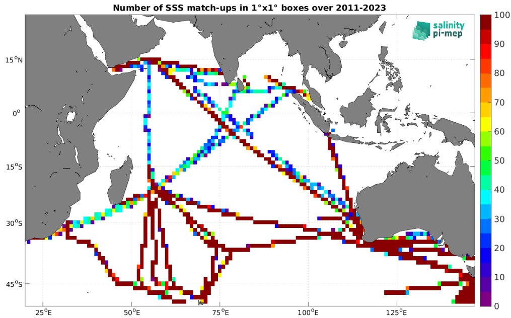
Figure 4: Number of SSS match-ups between TSG (LEGOS-DM) SSS and the SMAP SSS L4 OI v2 - Monthly (IPRC) SSS product for the Indian Ocean Pi-MEP region over 1^\circ \times 1^\circ boxes and for the full satellite product period.
