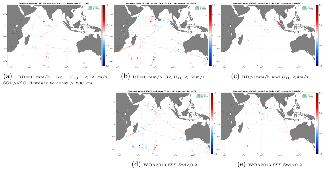
Figure 12: Temporal mean gridded over spatial boxes of size 1^\circ \times 1^\circ of \Delta SSS (SMAP SSS L4 OI v2 - Monthly (IPRC) - TSG (LEGOS-DM)) for 5 different subdatasets corresponding to:RR=0 mm/h, 3 < U_{10} < 12 m/s, SST > 5^\circ\text{C} , distance to coast > 800 km (a), RR=0 mm/h, 3 < U_{10} < 12 m/s (b), RR > 1 mm/h and U_{10} < 4 m/s (c), WOA2013 SSS Std < 0.2 (d), WOA2013 SSS Std > 0.2 (e).
