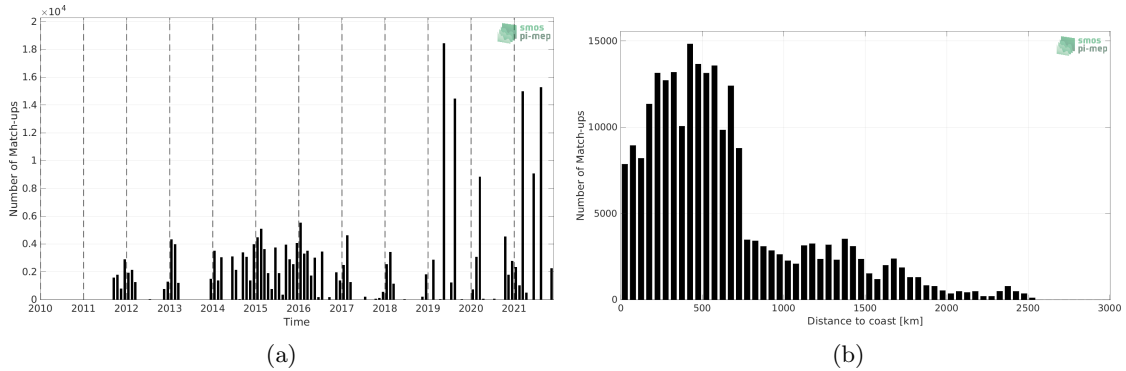
Figure 1: Number of match-ups between TSG (LEGOS-DM) and SMAP SSS L4 OI v2 - Monthly (IPRC) SSS as a function of time (a) and as function of the distance to coast (b) over the Indian Ocean Pi-MEP region and for the full satellite product period.
