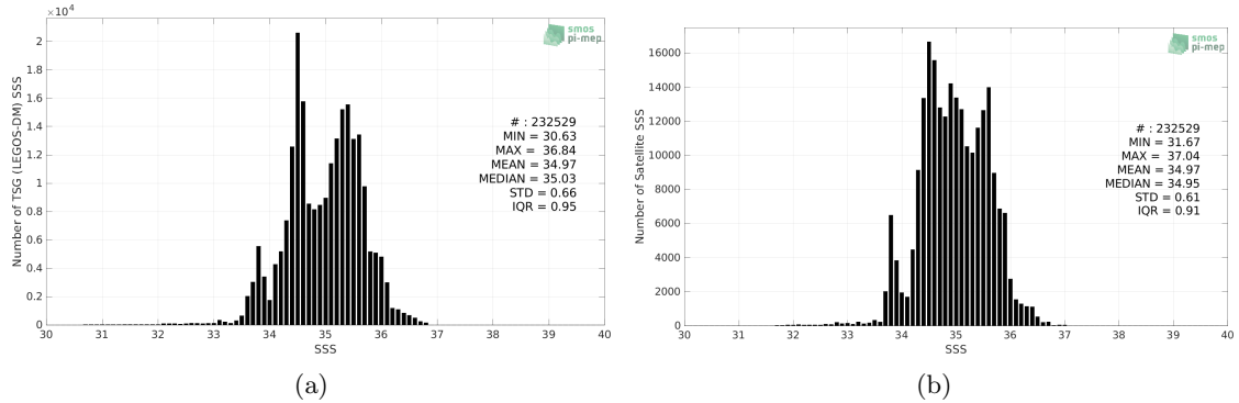
Figure 2: Histograms of SSS from TSG (LEGOS-DM) (a) and SMAP SSS L4 OI v2 - Monthly (IPRC) (b) considering all match-up pairs per bins of 0.1 over the Indian Ocean Pi-MEP region and for the full satellite product period.
