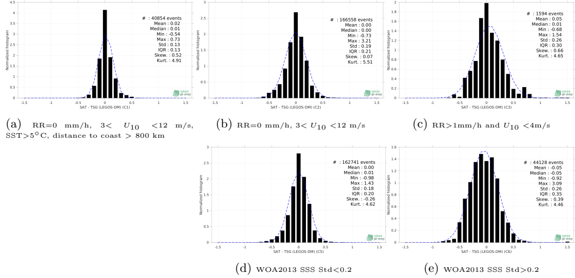
Figure 13: Normalized histogram of \Delta SSS (SMAP SSS L4 OI v2 - Monthly (IPRC) - TSG (LEGOS-DM)) for 5 different subdatasets corresponding to: RR=0 mm/h, 3 < U_{10} < 12 m/s, SST>5°C, distance to coast > 800 km (a), RR=0 mm/h, 3 < U_{10} < 12 m/s (b), RR>1mm/h and U_{10} < 4 m/s (c), WOA2013 SSS Std<0.2 (d), WOA2013 SSS Std>0.2 (e).
