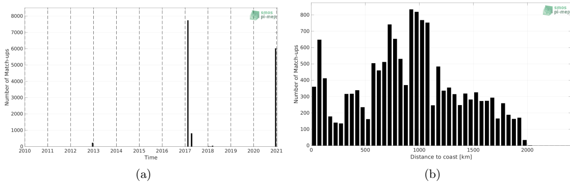
Figure 1: Number of match-ups between TSG (GOSUD-Sailing-ship) and SMAP SSS L4 OI v2 - Monthly (IPRC) SSS as a function of time (a) and as function of the distance to coast (b) over the Indian Ocean Pi-MEP region and for the full satellite product period.
