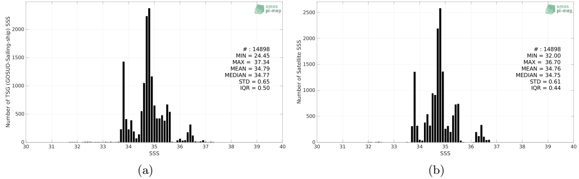
Figure 2: Histograms of SSS from TSG (GOSUD-Sailing-ship) (a) and SMAP SSS L4 OI v2 - Monthly (IPRC) (b) considering all match-up pairs per bins of 0.1 over the Indian Ocean Pi-MEP region and for the full satellite product period.
