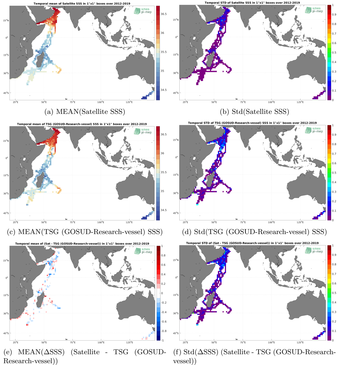
Figure 6: Temporal mean (left) and Std (right) of SSS from SMAP SSS L4 OI v2 - Monthly (IPRC) (top), TSG (GOSUD-Research-vessel) (middle), and of \Delta SSS (Satellite - TSG (GOSUD-Research-vessel)). Only match-up pairs are used to generate these maps.
