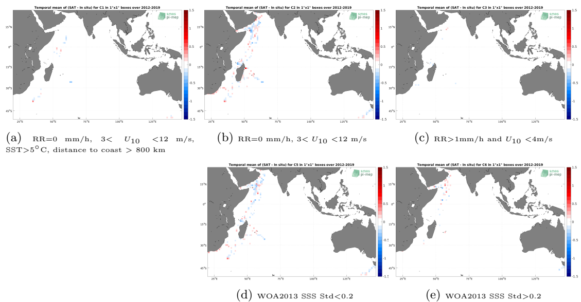
Figure 12: Temporal mean gridded over spatial boxes of size 1^\circ \times 1^\circ of \Delta SSS (SMAP SSS L4 OI v2 - Monthly (IPRC) - TSG (GOSUD-Research-vessel)) for 5 different subdatasets corresponding to: RR=0 mm/h, 3 < U_{10} < 12 m/s, SST > 5°C, distance to coast > 800 km (a), RR=0 mm/h, 3 < U_{10} < 12 m/s (b), RR > 1mm/h and U_{10} < 4 m/s (c), WOA2013 SSS Std < 0.2 (d), WOA2013 SSS Std > 0.2 (e).
