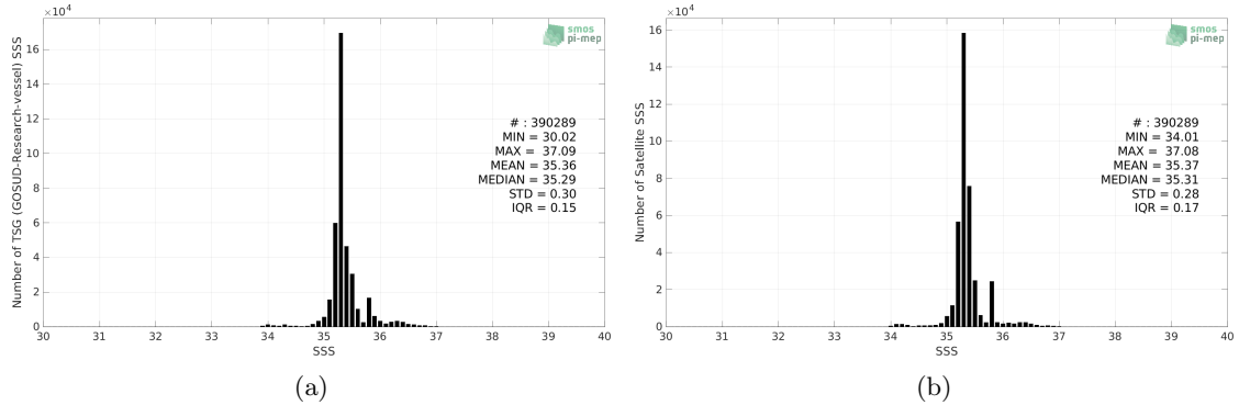
Figure 2: Histograms of SSS from TSG (GOSUD-Research-vessel) (a) and SMAP SSS L4 OI v2 - Monthly (IPRC) (b) considering all match-up pairs per bins of 0.1 over the Indian Ocean Pi-MEP region and for the full satellite product period.
