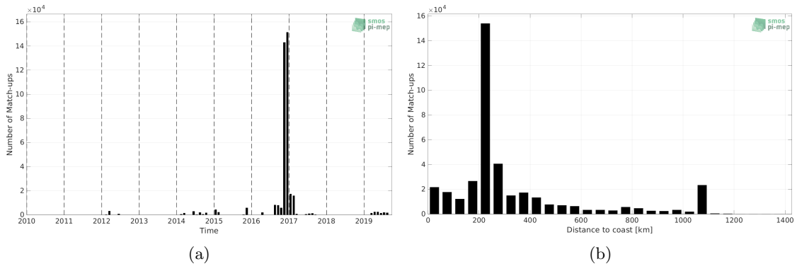
Figure 1: Number of match-ups between TSG (GOSUD-Research-vessel) and SMAP SSS L4 OI v2 - Monthly (IPRC) SSS as a function of time (a) and as function of the distance to coast (b) over the Indian Ocean Pi-MEP region and for the full satellite product period.
