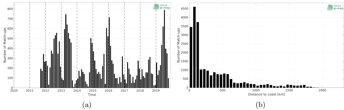
Figure 1: Number of match-ups between Marine mammals and SMAP SSS L4 OI v2 - Monthly (IPRC) SSS as a function of time (a) and as function of the distance to coast (b) over the Indian Ocean Pi-MEP region and for the full satellite product period.
