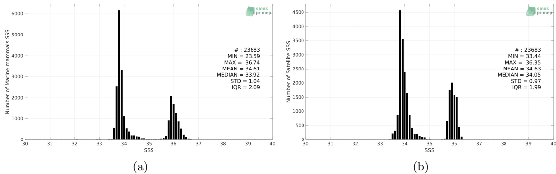
Figure 2: Histograms of SSS from Marine mammals (a) and SMAP SSS L4 OI v2 - Monthly (IPRC) (b) considering all match-up pairs per bins of 0.1 over the Indian Ocean Pi-MEP region and for the full satellite product period.
