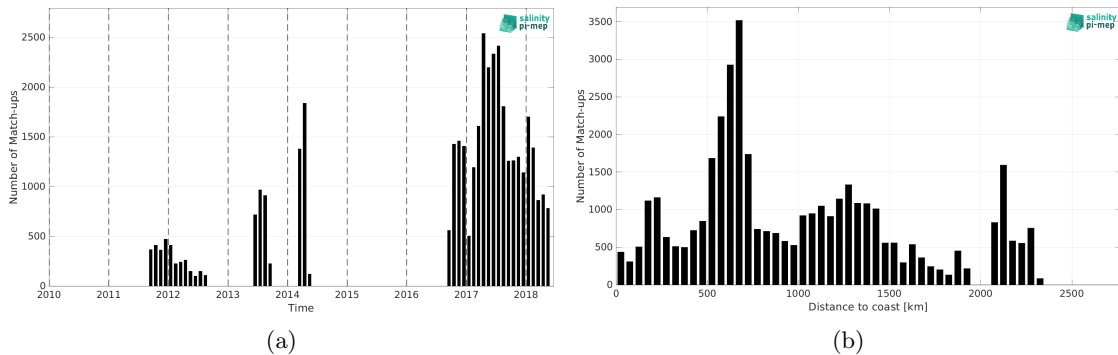
Figure 1: Number of match-ups between Surface drifters and SMAP SSS L4 OI v2 - Monthly (IPRC) SSS as a function of time (a) and as function of the distance to coast (b) over the Indian Ocean Pi-MEP region and for the full satellite product period.
