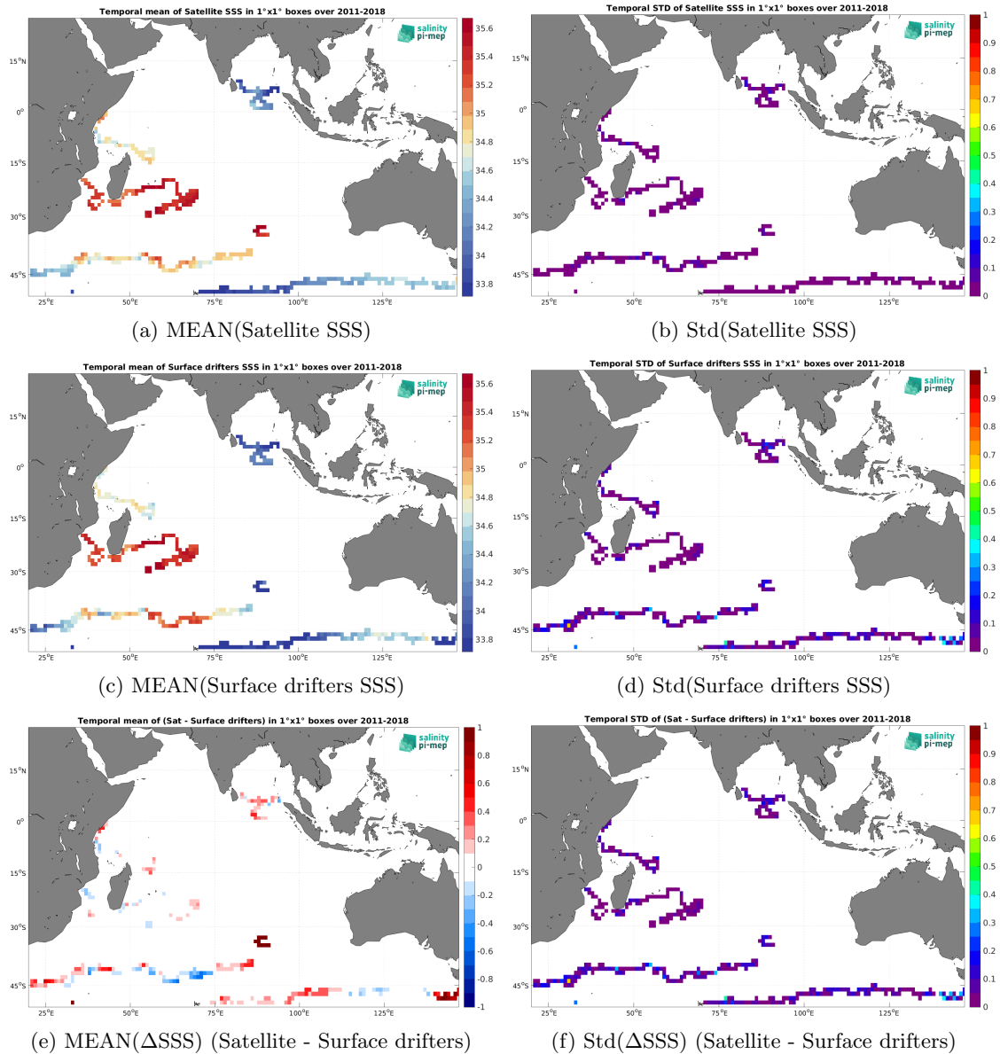
Figure 5: Temporal mean (left) and Std (right) of SSS from SMAP SSS L4 OI v2 - Monthly (IPRC) (top), Surface drifters (middle), and of \Delta SSS (Satellite - Surface drifters). Only match-up pairs are used to generate these maps.
