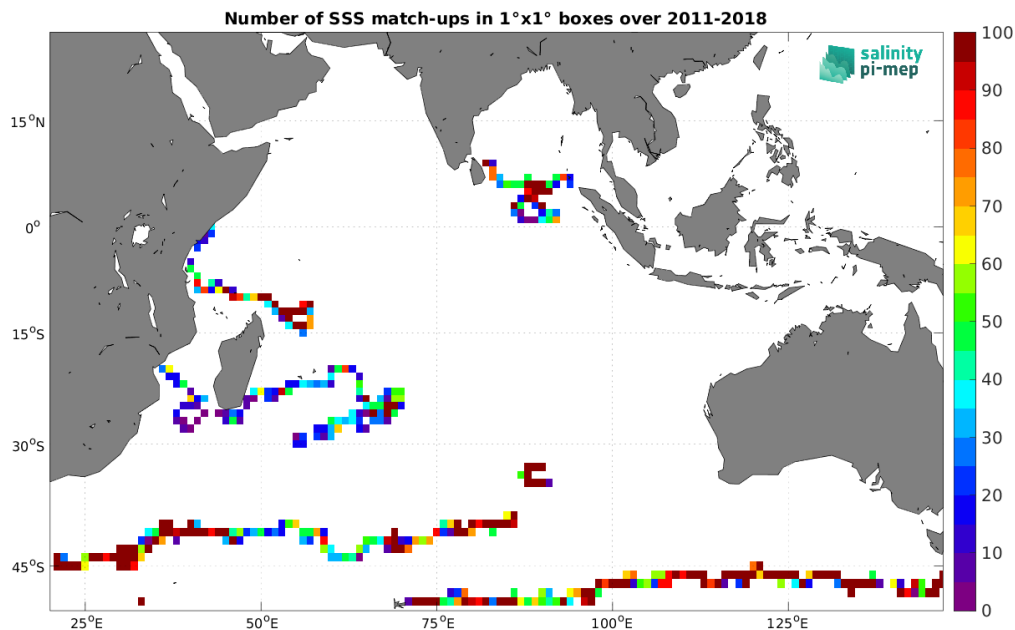
Figure 3: Number of SSS match-ups between Surface drifters SSS and the SMAP SSS L4 OI v2 - Monthly (IPRC) SSS product for the Indian Ocean Pi-MEP region over 1^\circ \times 1^\circ boxes and for the full satellite product period.
