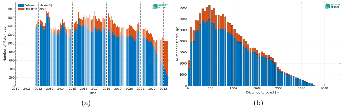
Figure 1: Number of match-ups between Argo and SMAP SSS L4 OI v2 - Monthly (IPRC) SSS as a function of time (a) and as function of the distance to coast (b) over the Indian Ocean Pi-MEP region and for the full satellite product period.
