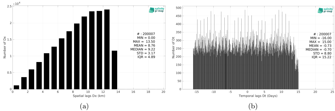
Figure 5: Histograms of the spatial (a) and temporal (b) lags between the location/time of the Argo measurement and the date of the corresponding SMAP SSS L4 OI v2 - Monthly (IPRC) SSS pixel.
