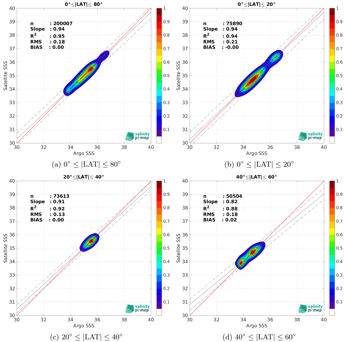
Figure 9: Contour maps of the concentration of SMAP SSS L4 OI v2 - Monthly (IPRC) SSS (y-axis) versus Argo SSS (x-axis) at match-up pairs for different latitude bands. For each plot, the red line shows x=y . The black thin and dashed lines indicate a linear fit through the data cloud and the \pm 95\% confidence levels, respectively. The number match-up pairs n , the slope and R^2 coefficient of the linear fit, the root mean square (RMS) and the mean bias between satellite and in situ data are indicated for each latitude band in each plots.
