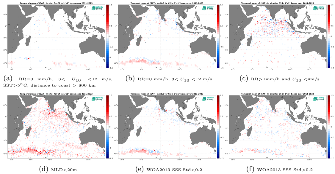
Figure 12: Temporal mean gridded over spatial boxes of size 1^\circ \times 1^\circ of \Delta SSS (SMAP SSS L4 OI v2 - Monthly (IPRC) - Argo) for 6 different subdatasets corresponding to:RR=0 mm/h, 3 < U_{10} < 12 m/s, SST >5^\circ C, distance to coast > 800 km (a), RR=0 mm/h, 3 < U_{10} < 12 m/s (b), RR >1 mm/h and U_{10} < 4 m/s (c),MLD <20 m (d),WOA2013 SSS Std <0.2 (e),WOA2013 SSS Std >0.2 (f).
