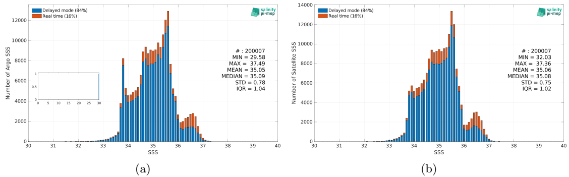
Figure 2: Histograms of SSS from Argo (a) and SMAP SSS L4 OI v2 - Monthly (IPRC) (b) considering all match-up pairs per bins of 0.1 over the Indian Ocean Pi-MEP region and for the full satellite product period.
