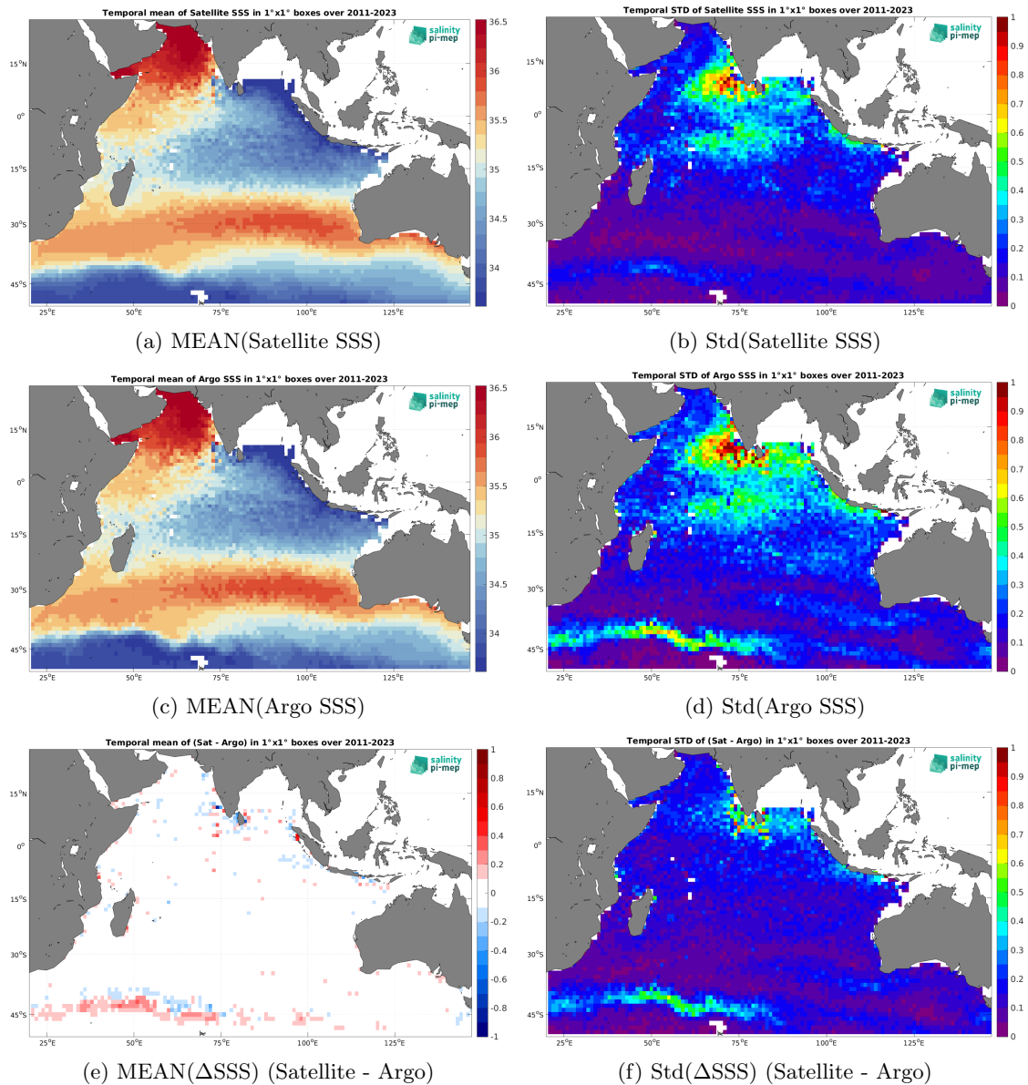
Figure 6: Temporal mean (left) and Std (right) of SSS from SMAP SSS L4 OI v2 - Monthly (IPRC) (top), Argo (middle), and of \Delta SSS (Satellite - Argo). Only match-up pairs are used to generate these maps.
