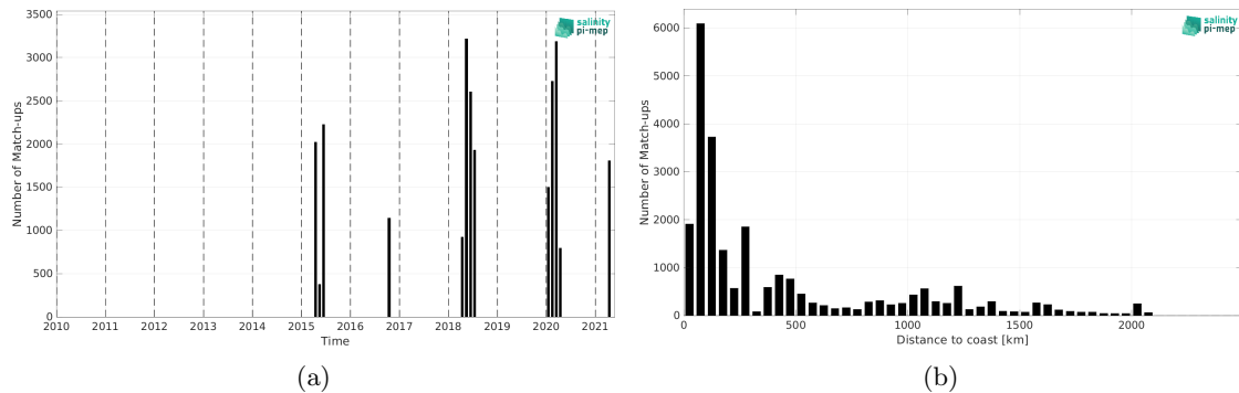
Figure 2: Number of match-ups between TSG (SAMOS) and SMAP SSS L3 v6 - 8-Day running (RSS) SSS as a function of time (a) and as function of the distance to coast (b) over the Indian Ocean Pi-MEP region and for the full satellite product period.
