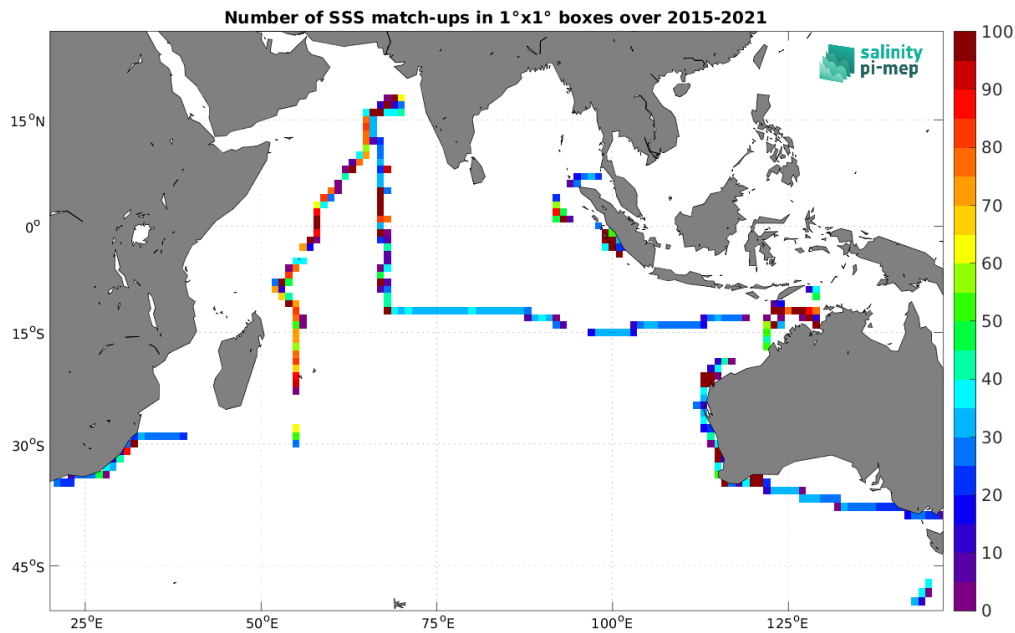
Figure 5: Number of SSS match-ups between TSG (SAMOS) SSS and the SMAP SSS L3 v6 - 8-Day running (RSS) SSS product for the Indian Ocean Pi-MEP region over 1^\circ \times 1^\circ boxes and for the full satellite product period.
