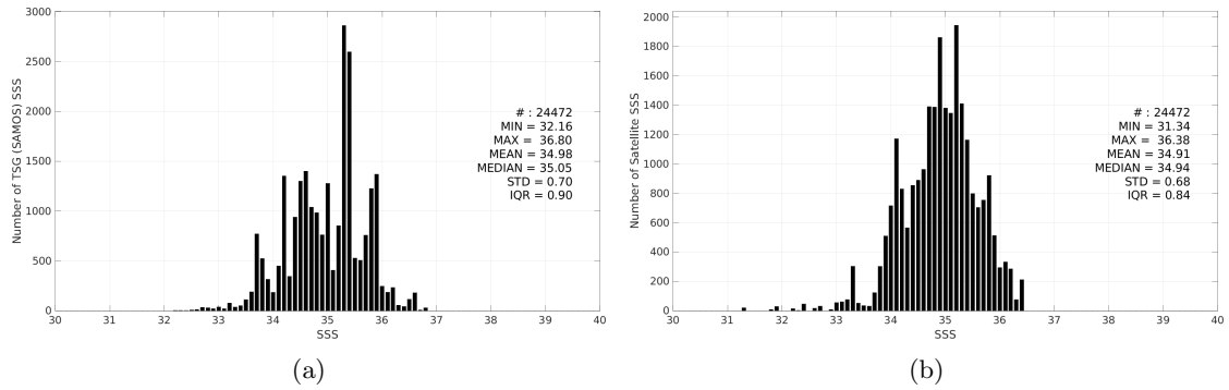
Figure 3: Histograms of SSS from TSG (SAMOS) (a) and SMAP SSS L3 v6 - 8-Day running (RSS) (b) considering all match-up pairs per bins of 0.1 over the Indian Ocean Pi-MEP region and for the full satellite product period.
