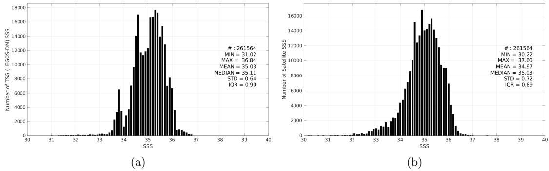
Figure 3: Histograms of SSS from TSG (LEGOS-DM) (a) and SMAP SSS L3 v6 - 8-Day running (RSS) (b) considering all match-up pairs per bins of 0.1 over the Indian Ocean Pi-MEP region and for the full satellite product period.
