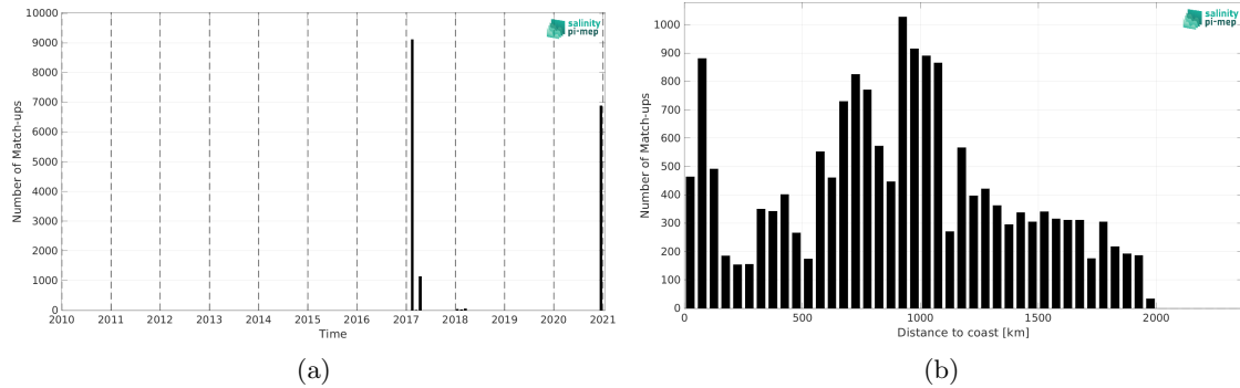
Figure 2: Number of match-ups between TSG (GOSUD-Sailing-ship) and SMAP SSS L3 v6 - 8-Day running (RSS) SSS as a function of time (a) and as function of the distance to coast (b) over the Indian Ocean Pi-MEP region and for the full satellite product period.
