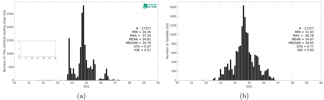
Figure 3: Histograms of SSS from TSG (GOSUD-Sailing-ship) (a) and SMAP SSS L3 v6 - 8-Day running (RSS) (b) considering all match-up pairs per bins of 0.1 over the Indian Ocean Pi-MEP region and for the full satellite product period.
