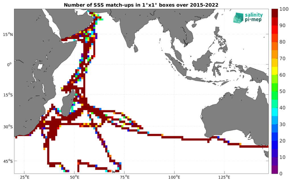
Figure 5: Number of SSS match-ups between TSG (GOSUD-Research-vessel) SSS and the SMAP SSS L3 v6 - 8-Day running (RSS) SSS product for the Indian Ocean Pi-MEP region over 1^\circ \times 1^\circ boxes and for the full satellite product period.
