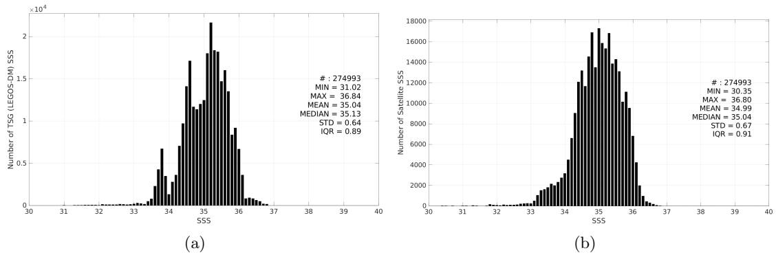
Figure 3: Histograms of SSS from TSG (LEGOS-DM) (a) and SMAP SSS L3 v6 - Monthly (RSS) (b) considering all match-up pairs per bins of 0.1 over the Indian Ocean Pi-MEP region and for the full satellite product period.
