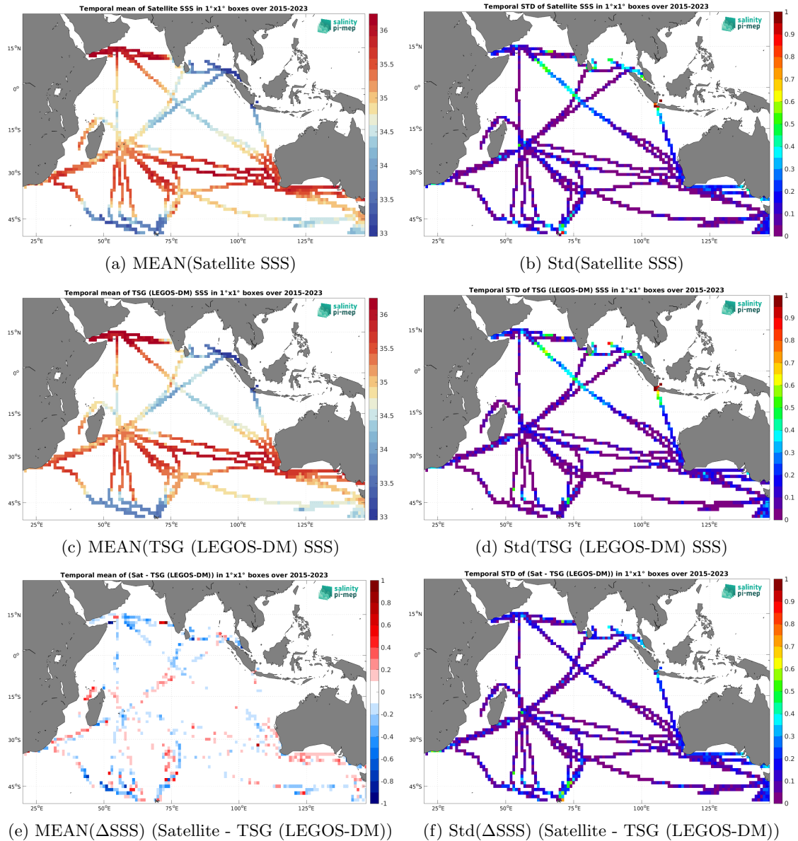
Figure 7: Temporal mean (left) and Std (right) of SSS from SMAP SSS L3 v6 - Monthly (RSS) (top), TSG (LEGOS-DM) (middle), and of \Delta SSS (Satellite - TSG (LEGOS-DM)). Only match-up pairs are used to generate these maps.
