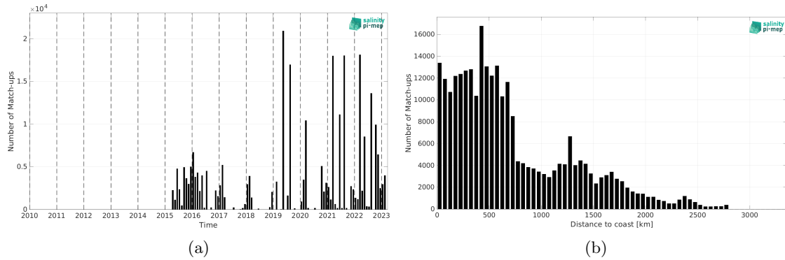
Figure 2: Number of match-ups between TSG (LEGOS-DM) and SMAP SSS L3 v6 - Monthly (RSS) SSS as a function of time (a) and as function of the distance to coast (b) over the Indian Ocean Pi-MEP region and for the full satellite product period.
