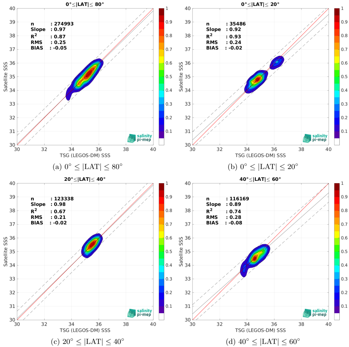
Figure 10: Contour maps of the concentration of SMAP SSS L3 v6 - Monthly (RSS) SSS (y-axis) versus TSG (LEGOS-DM) SSS (x-axis) at match-up pairs for different latitude bands. For each plot, the red line shows x=y . The black thin and dashed lines indicate a linear fit through the data cloud and the \pm 95\% confidence levels, respectively. The number match-up pairs n , the slope and R^2 coefficient of the linear fit, the root mean square (RMS) and the mean bias between satellite and in situ data are indicated for each latitude band in each plots.
