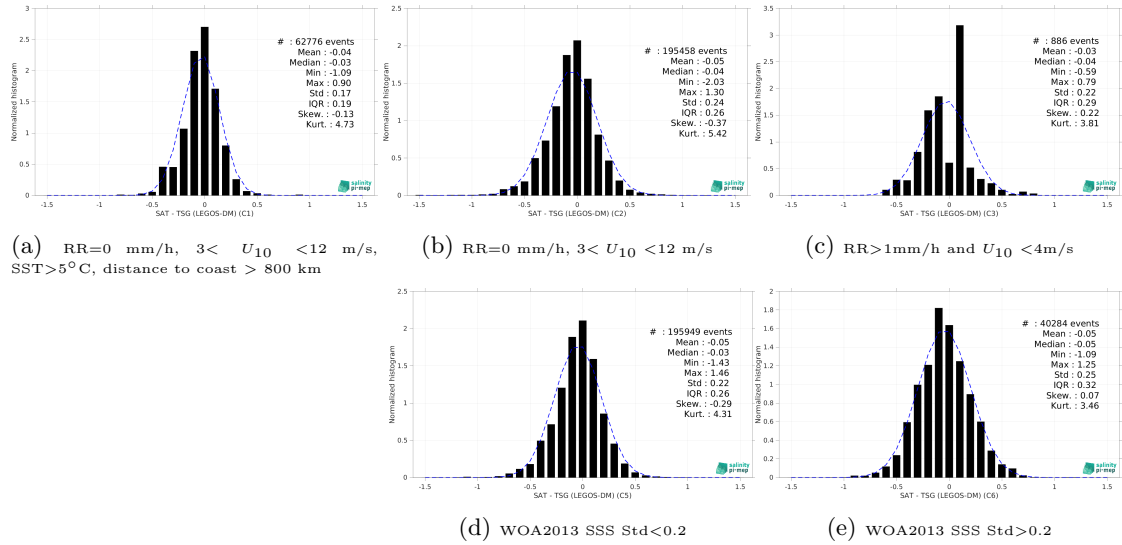
Figure 15: Normalized histogram of \Delta SSS (SMAP SSS L3 v6 - Monthly (RSS) - TSG (LEGOS-DM)) for 5 different subdatasets corresponding to: RR=0 mm/h, 3 < U_{10} < 12 m/s, SST > 5°C, distance to coast > 800 km (a), RR=0 mm/h, 3 < U_{10} < 12 m/s (b), RR > 1mm/h and U_{10} < 4 m/s (c), WOA2013 SSS Std < 0.2 (d), WOA2013 SSS Std > 0.2 (e).
