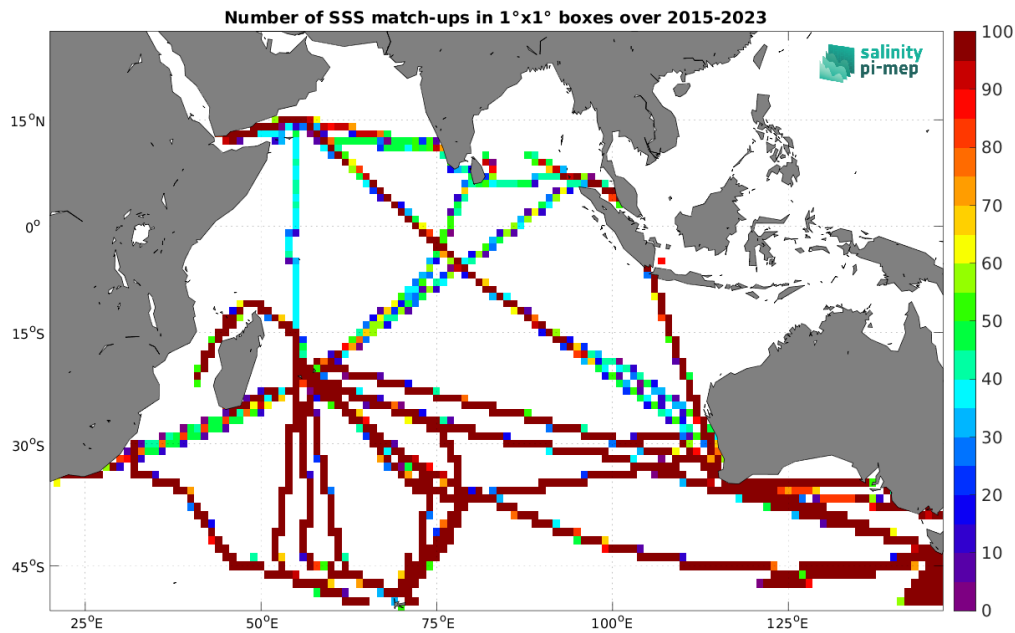
Figure 5: Number of SSS match-ups between TSG (LEGOS-DM) SSS and the SMAP SSS L3 v6 - Monthly (RSS) SSS product for the Indian Ocean Pi-MEP region over 1^\circ \times 1^\circ boxes and for the full satellite product period.
