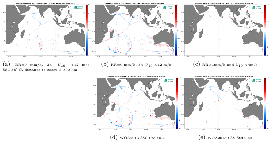
Figure 14: Temporal mean gridded over spatial boxes of size 1^\circ \times 1^\circ of \Delta SSS (SMAP SSS L3 v6 - Monthly (RSS) - TSG (LEGOS-DM)) for 5 different subdatasets corresponding to:RR=0 mm/h, 3 < U_{10} < 12 m/s, SST >5^\circ C, distance to coast > 800 km (a), RR=0 mm/h, 3 < U_{10} < 12 m/s (b), RR >1 mm/h and U_{10} < 4 m/s (c), WOA2013 SSS Std <0.2 (d), WOA2013 SSS Std >0.2 (e).
