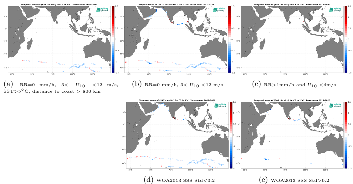
Figure 14: Temporal mean gridded over spatial boxes of size 1^\circ \times 1^\circ of \Delta SSS (SMAP SSS L3 v6 - Monthly (RSS) - TSG (GOSUD-Sailing-ship)) for 5 different subdatasets corresponding to:RR=0 mm/h, 3 < U_{10} < 12 m/s, SST >5^\circ C, distance to coast > 800 km (a), RR=0 mm/h, 3 < U_{10} < 12 m/s (b), RR >1 mm/h and U_{10} < 4 m/s (c), WOA2013 SSS Std <0.2 (d), WOA2013 SSS Std >0.2 (e).
