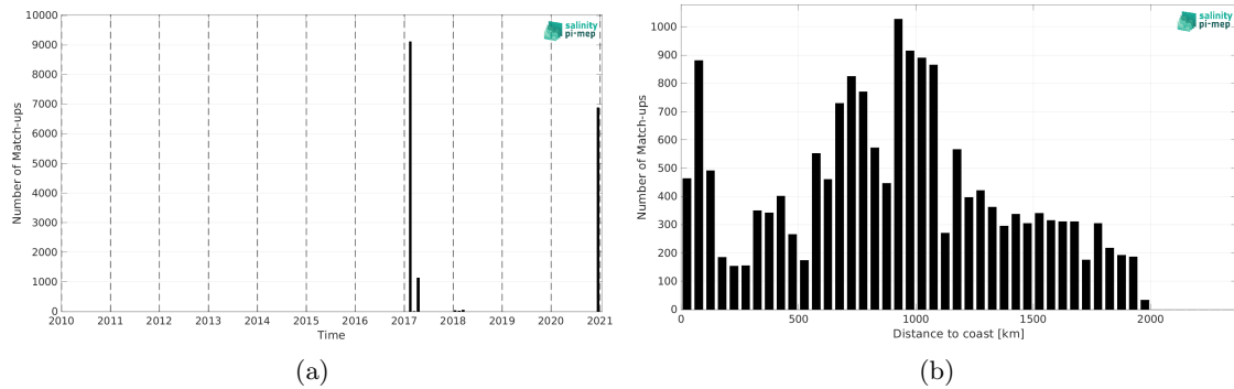
Figure 2: Number of match-ups between TSG (GOSUD-Sailing-ship) and SMAP SSS L3 v6 - Monthly (RSS) SSS as a function of time (a) and as function of the distance to coast (b) over the Indian Ocean Pi-MEP region and for the full satellite product period.
