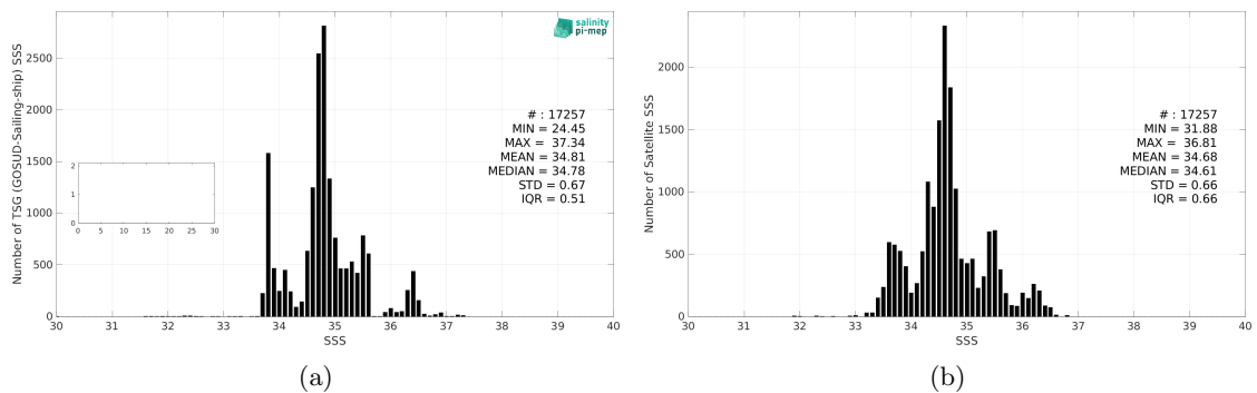
Figure 3: Histograms of SSS from TSG (GOSUD-Sailing-ship) (a) and SMAP SSS L3 v6 - Monthly (RSS) (b) considering all match-up pairs per bins of 0.1 over the Indian Ocean Pi-MEP region and for the full satellite product period.
