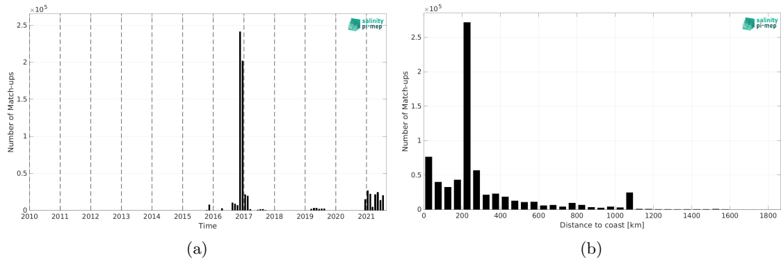
Figure 2: Number of match-ups between TSG (GOSUD-Research-vessel) and SMAP SSS L3 v6 - Monthly (RSS) SSS as a function of time (a) and as function of the distance to coast (b) over the Indian Ocean Pi-MEP region and for the full satellite product period.
