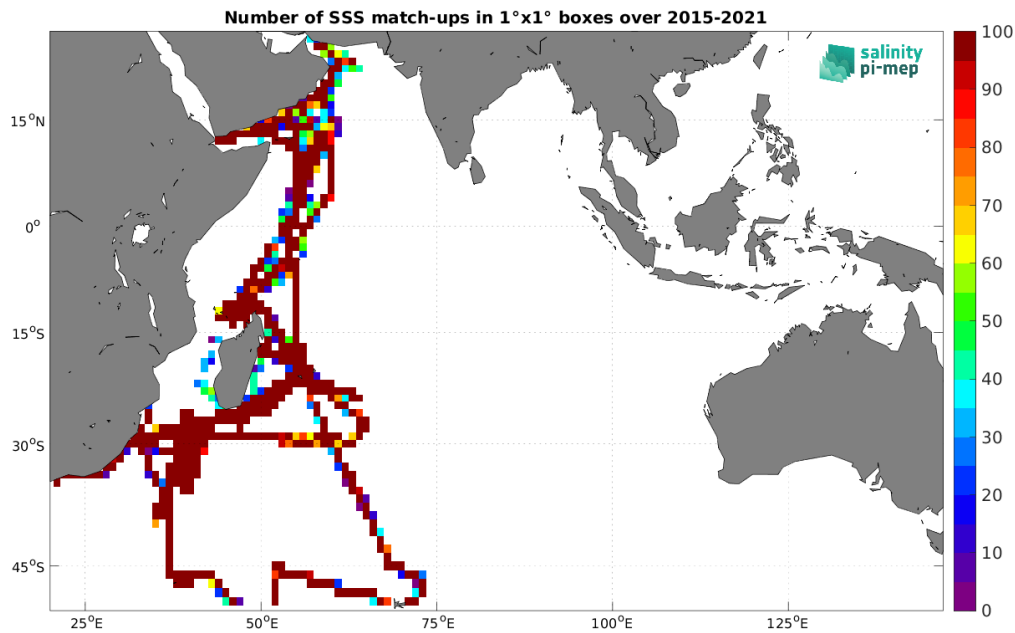
Figure 5: Number of SSS match-ups between TSG (GOSUD-Research-vessel) SSS and the SMAP SSS L3 v6 - Monthly (RSS) SSS product for the Indian Ocean Pi-MEP region over 1^\circ \times 1^\circ boxes and for the full satellite product period.
