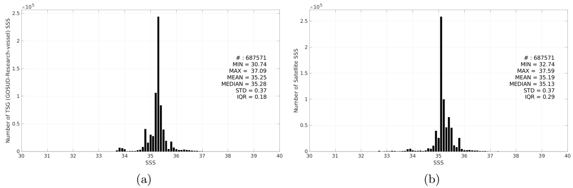
Figure 3: Histograms of SSS from TSG (GOSUD-Research-vessel) (a) and SMAP SSS L3 v6 - Monthly (RSS) (b) considering all match-up pairs per bins of 0.1 over the Indian Ocean Pi-MEP region and for the full satellite product period.
