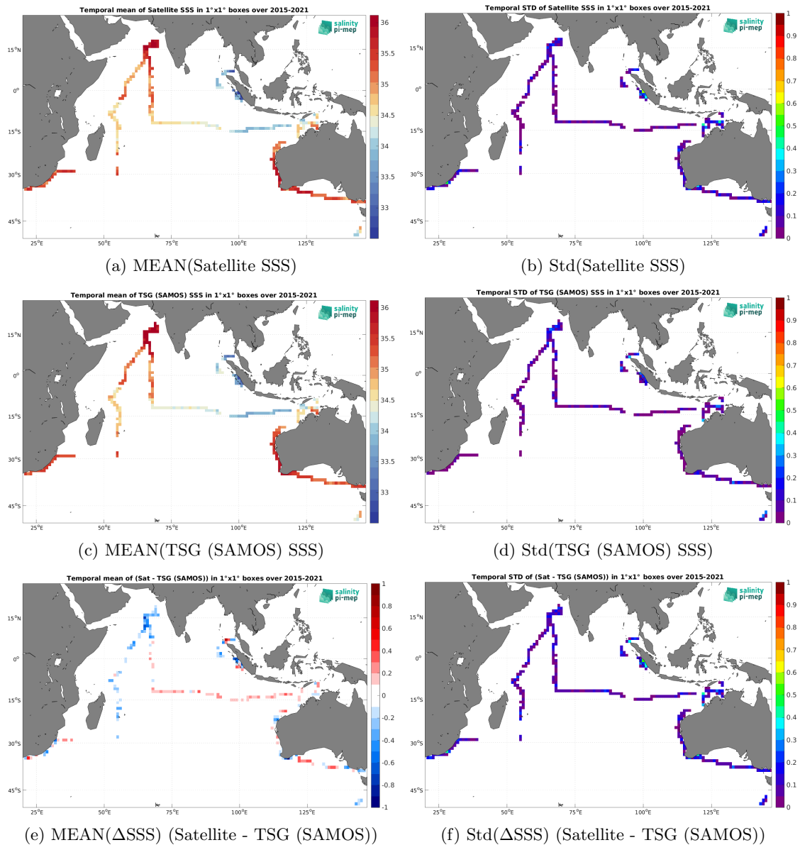
Figure 7: Temporal mean (left) and Std (right) of SSS from SMAP SSS L3 v5.3 - 8-Day running (RSS) (top), TSG (SAMOS) (middle), and of \Delta SSS (Satellite - TSG (SAMOS)). Only match-up pairs are used to generate these maps.
