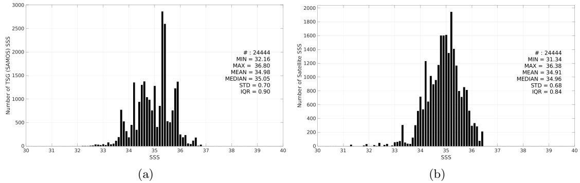
Figure 3: Histograms of SSS from TSG (SAMOS) (a) and SMAP SSS L3 v5.3 - 8-Day running (RSS) (b) considering all match-up pairs per bins of 0.1 over the Indian Ocean Pi-MEP region and for the full satellite product period.
