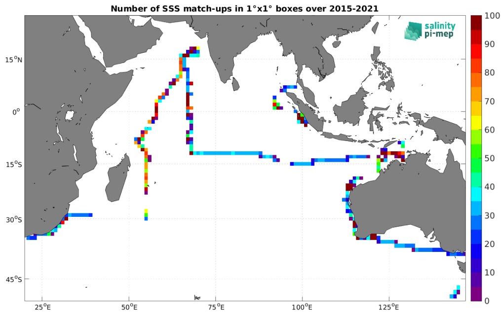
Figure 5: Number of SSS match-ups between TSG (SAMOS) SSS and the SMAP SSS L3 v5.3 - 8-Day running (RSS) SSS product for the Indian Ocean Pi-MEP region over 1^\circ \times 1^\circ boxes and for the full satellite product period.
