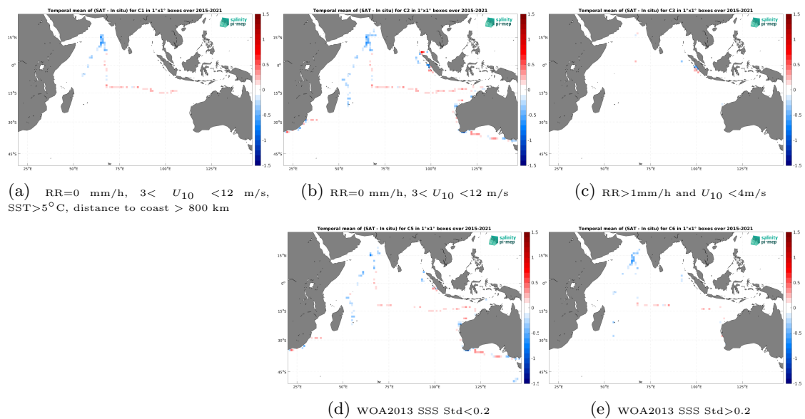
Figure 14: Temporal mean gridded over spatial boxes of size 1^\circ \times 1^\circ of \Delta SSS (SMAP SSS L3 v5.3 - 8-Day running (RSS) - TSG (SAMOS)) for 5 different subdatasets corresponding to:RR=0 mm/h, 3 < U_{10} < 12 m/s, SST >5^\circ\text{C} , distance to coast > 800 km (a), RR=0 mm/h, 3 < U_{10} < 12 m/s (b), RR >1 mm/h and U_{10} < 4 m/s (c), WOA2013 SSS Std <0.2 (d), WOA2013 SSS Std >0.2 (e).
