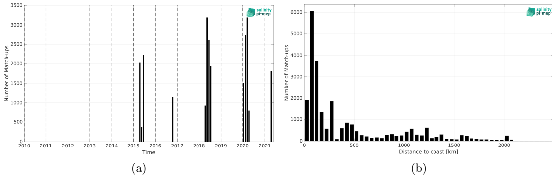
Figure 2: Number of match-ups between TSG (SAMOS) and SMAP SSS L3 v5.3 - 8-Day running (RSS) SSS as a function of time (a) and as function of the distance to coast (b) over the Indian Ocean Pi-MEP region and for the full satellite product period.
