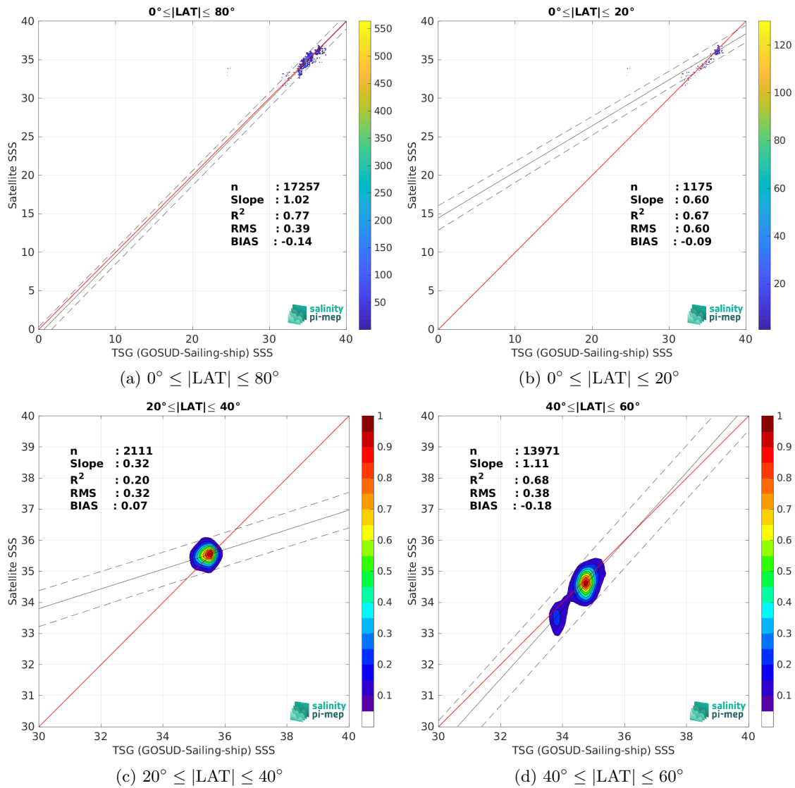
Figure 10: Contour maps of the concentration of SMAP SSS L3 v5.3 - 8-Day running (RSS) SSS (y-axis) versus TSG (GOSUD-Sailing-ship) SSS (x-axis) at match-up pairs for different latitude bands. For each plot, the red line shows x=y . The black thin and dashed lines indicate a linear fit through the data cloud and the \pm 95\% confidence levels, respectively. The number match-up pairs n , the slope and R^2 coefficient of the linear fit, the root mean square (RMS) and the mean bias between satellite and in situ data are indicated for each latitude band in each plots.
