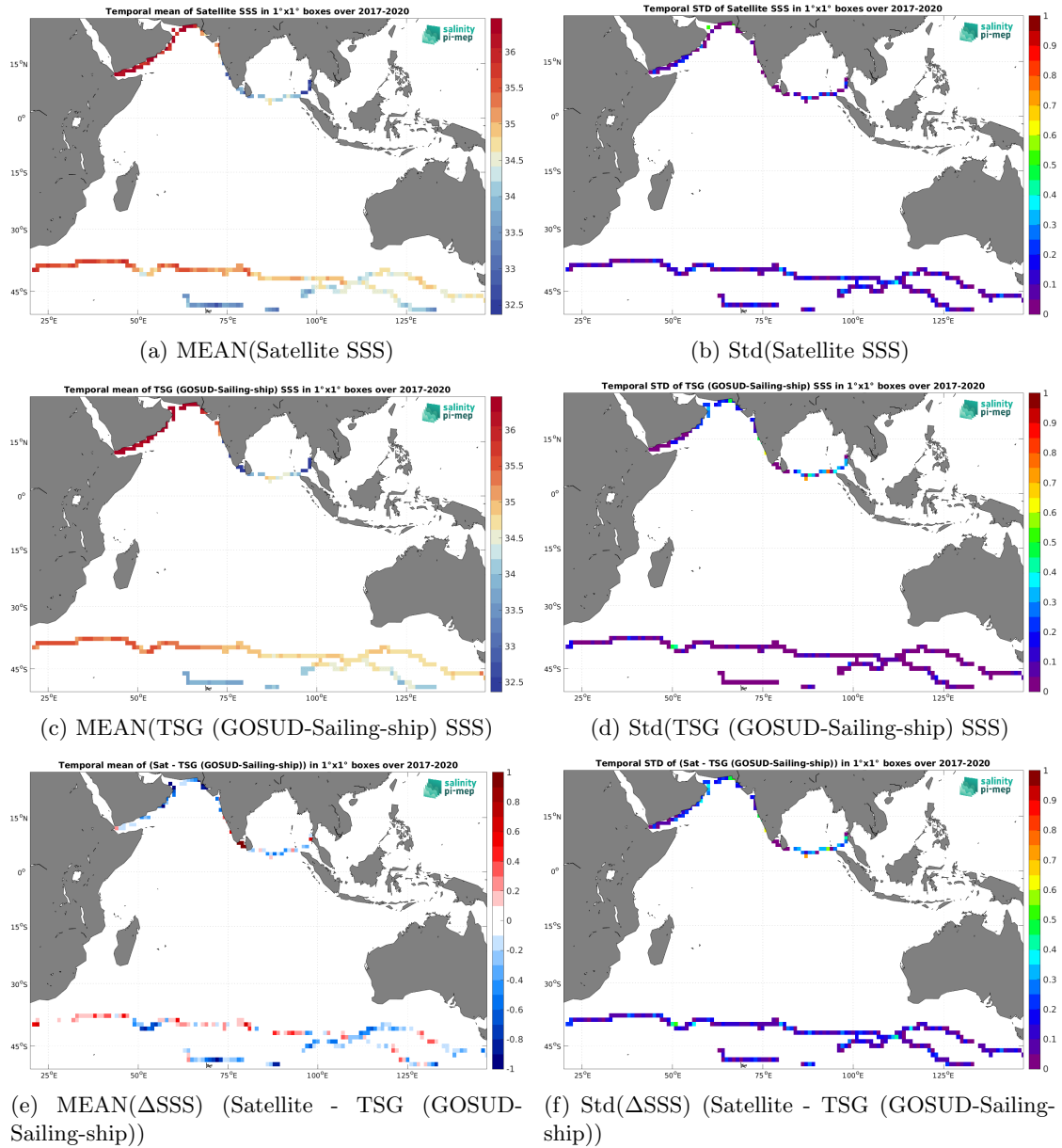
Figure 7: Temporal mean (left) and Std (right) of SSS from SMAP SSS L3 v5.3 - 8-Day running (RSS) (top), TSG (GOSUD-Sailing-ship) (middle), and of \Delta SSS (Satellite - TSG (GOSUD-Sailing-ship)). Only match-up pairs are used to generate these maps.
