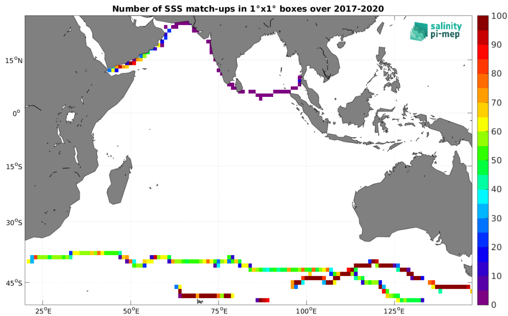
Figure 5: Number of SSS match-ups between TSG (GOSUD-Sailing-ship) SSS and the SMAP SSS L3 v5.3 - 8-Day running (RSS) SSS product for the Indian Ocean Pi-MEP region over 1^\circ \times 1^\circ boxes and for the full satellite product period.
