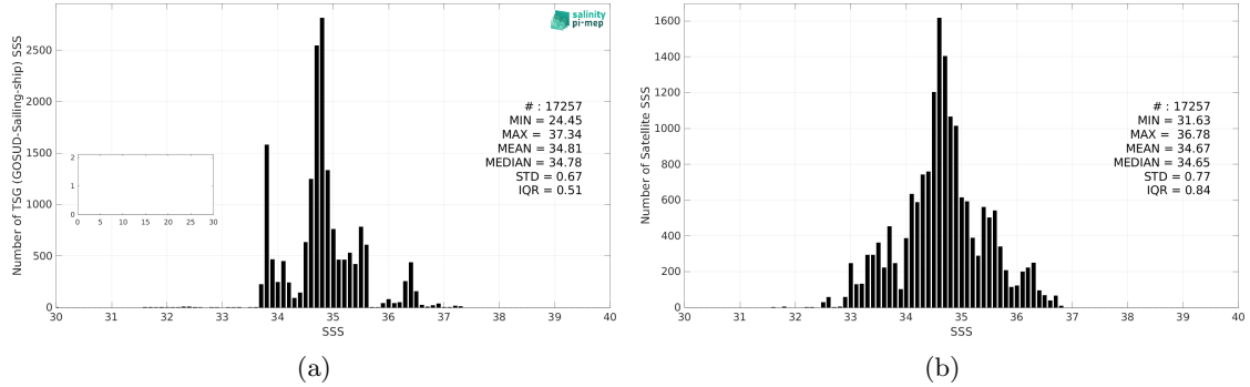
Figure 3: Histograms of SSS from TSG (GOSUD-Sailing-ship) (a) and SMAP SSS L3 v5.3 - 8-Day running (RSS) (b) considering all match-up pairs per bins of 0.1 over the Indian Ocean Pi-MEP region and for the full satellite product period.
