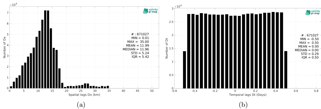
Figure 6: Histograms of the spatial (a) and temporal (b) lags between the location/time of the TSG (GOSUD-Research-vessel) measurement and the date of the corresponding SMAP SSS L3 v5.3 - 8-Day running (RSS) SSS pixel.
