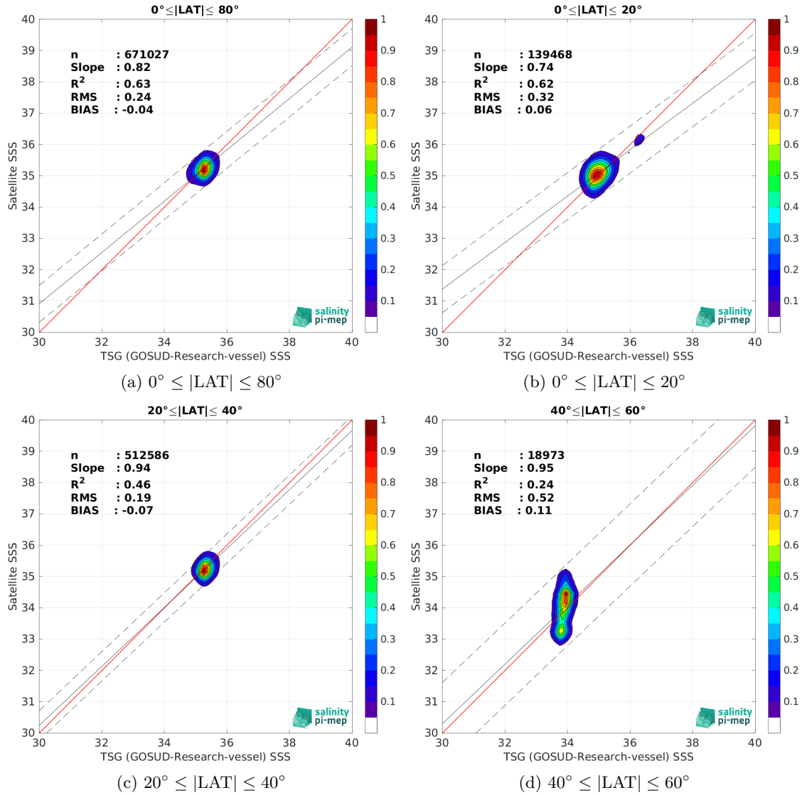
Figure 10: Contour maps of the concentration of SMAP SSS L3 v5.3 - 8-Day running (RSS) SSS (y-axis) versus TSG (GOSUD-Research-vessel) SSS (x-axis) at match-up pairs for different latitude bands. For each plot, the red line shows x=y . The black thin and dashed lines indicate a linear fit through the data cloud and the \pm 95\% confidence levels, respectively. The number match-up pairs n , the slope and R^2 coefficient of the linear fit, the root mean square (RMS) and the mean bias between satellite and in situ data are indicated for each latitude band in each plots.
