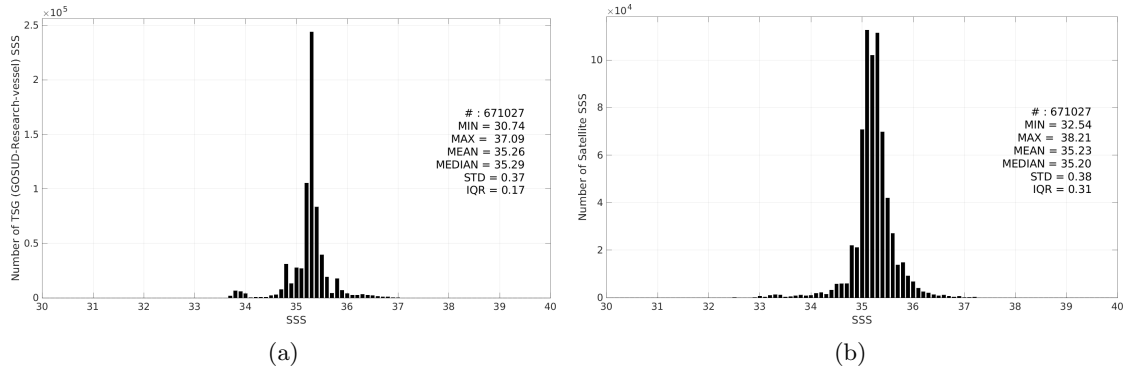
Figure 3: Histograms of SSS from TSG (GOSUD-Research-vessel) (a) and SMAP SSS L3 v5.3 - 8-Day running (RSS) (b) considering all match-up pairs per bins of 0.1 over the Indian Ocean Pi-MEP region and for the full satellite product period.
