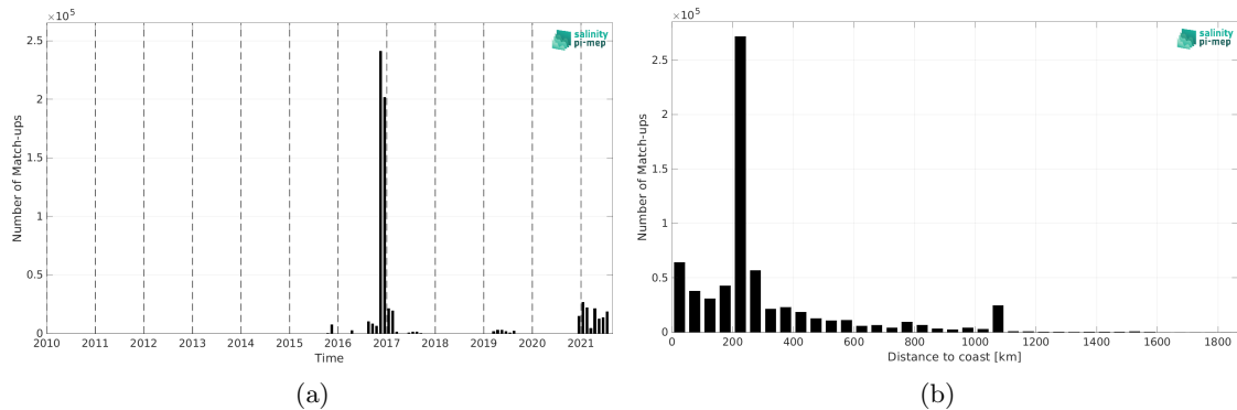
Figure 2: Number of match-ups between TSG (GOSUD-Research-vessel) and SMAP SSS L3 v5.3 - 8-Day running (RSS) SSS as a function of time (a) and as function of the distance to coast (b) over the Indian Ocean Pi-MEP region and for the full satellite product period.
