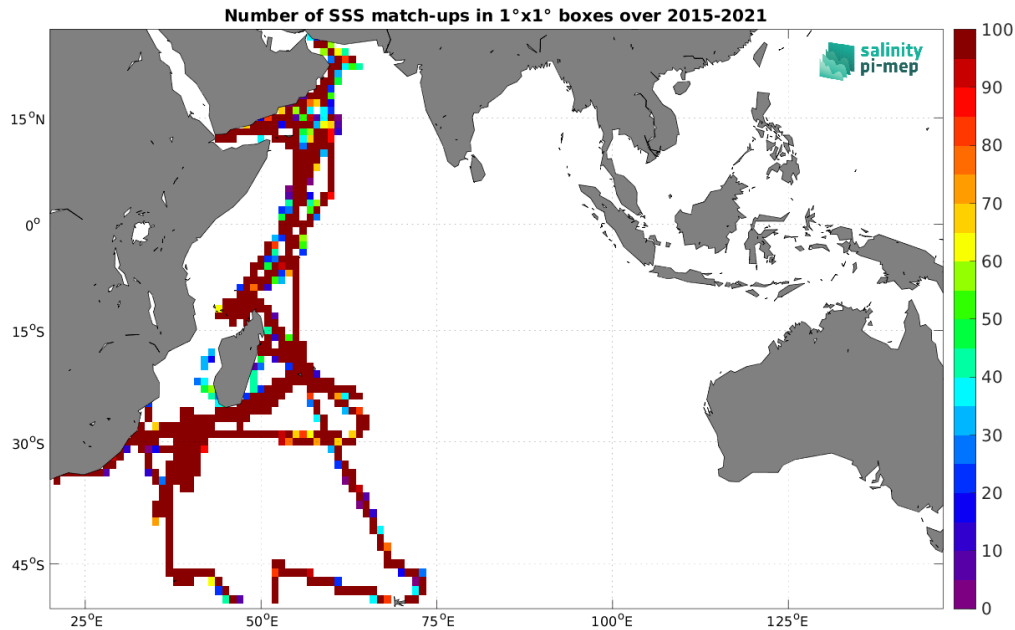
Figure 5: Number of SSS match-ups between TSG (GOSUD-Research-vessel) SSS and the SMAP SSS L3 v5.3 - 8-Day running (RSS) SSS product for the Indian Ocean Pi-MEP region over 1^\circ \times 1^\circ boxes and for the full satellite product period.
