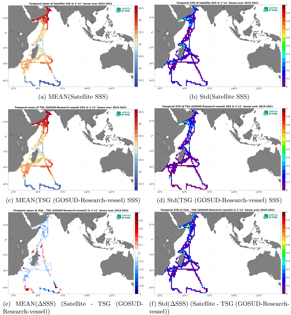
Figure 7: Temporal mean (left) and Std (right) of SSS from SMAP SSS L3 v5.3 - 8-Day running (RSS) (top), TSG (GOSUD-Research-vessel) (middle), and of \Delta SSS (Satellite - TSG (GOSUD-Research-vessel)). Only match-up pairs are used to generate these maps.
