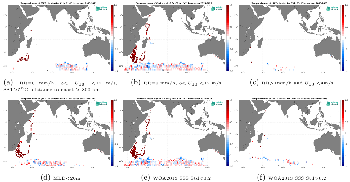
Figure 14: Temporal mean gridded over spatial boxes of size 1^\circ \times 1^\circ of \Delta\text{SSS} (SMAP SSS L3 v5.3 - 8-Day running (RSS) - Marine mammals) for 6 different subdatasets corresponding to: RR=0 mm/h, 3 < U_{10} < 12 m/s, SST > 5°C, distance to coast > 800 km (a), RR=0 mm/h, 3 < U_{10} < 12 m/s (b), RR > 1mm/h and U_{10} < 4 m/s (c), MLD < 20m (d), WOA2013 SSS Std < 0.2 (e), WOA2013 SSS Std > 0.2 (f).
