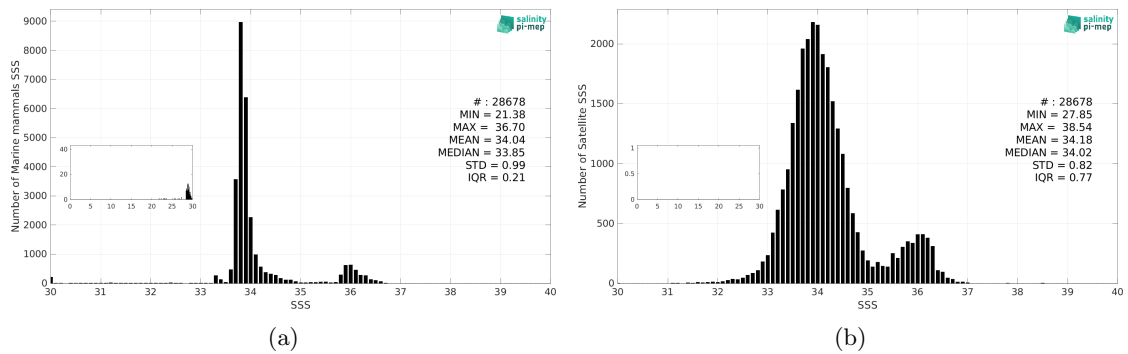
Figure 3: Histograms of SSS from Marine mammals (a) and SMAP SSS L3 v5.3 - 8-Day running (RSS) (b) considering all match-up pairs per bins of 0.1 over the Indian Ocean Pi-MEP region and for the full satellite product period.
