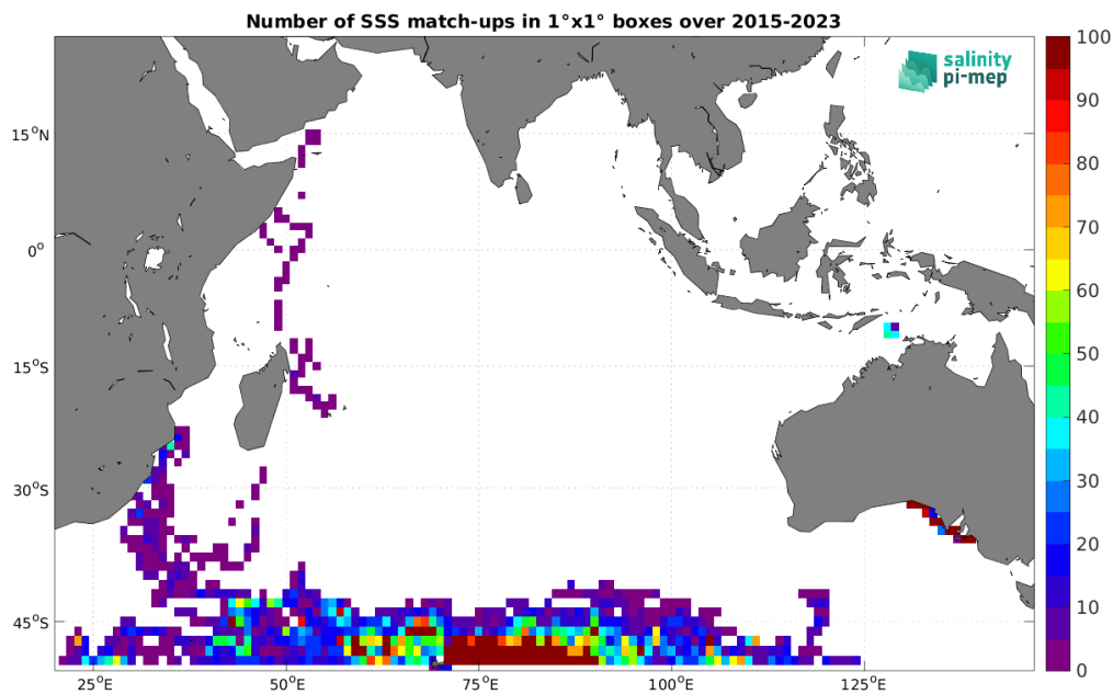
Figure 5: Number of SSS match-ups between Marine mammals SSS and the SMAP SSS L3 v5.3 - 8-Day running (RSS) SSS product for the Indian Ocean Pi-MEP region over 1^\circ \times 1^\circ boxes and for the full satellite product period.
