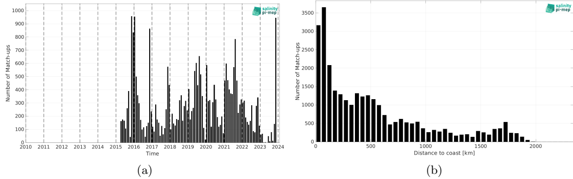
Figure 2: Number of match-ups between Marine mammals and SMAP SSS L3 v5.3 - 8-Day running (RSS) SSS as a function of time (a) and as function of the distance to coast (b) over the Indian Ocean Pi-MEP region and for the full satellite product period.
