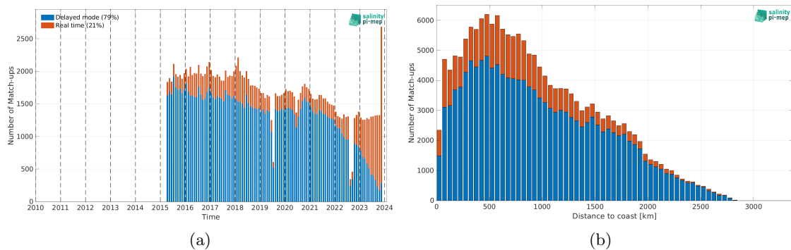
Figure 2: Number of match-ups between Argo and SMAP SSS L3 v5.3 - 8-Day running (RSS) SSS as a function of time (a) and as function of the distance to coast (b) over the Indian Ocean Pi-MEP region and for the full satellite product period.
