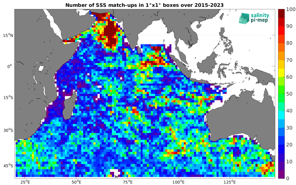
Figure 5: Number of SSS match-ups between Argo SSS and the SMAP SSS L3 v5.3 - 8-Day running (RSS) SSS product for the Indian Ocean Pi-MEP region over 1^\circ \times 1^\circ boxes and for the full satellite product period.
