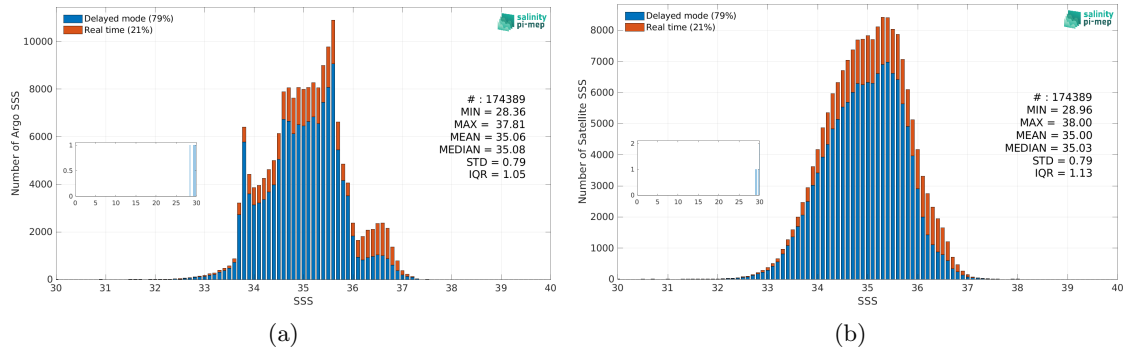
Figure 3: Histograms of SSS from Argo (a) and SMAP SSS L3 v5.3 - 8-Day running (RSS) (b) considering all match-up pairs per bins of 0.1 over the Indian Ocean Pi-MEP region and for the full satellite product period.
