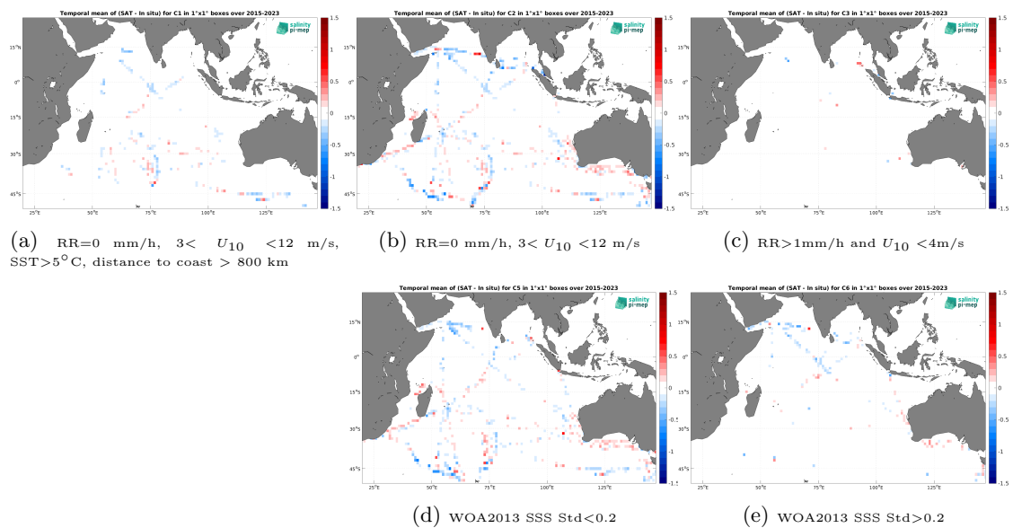
Figure 14: Temporal mean gridded over spatial boxes of size 1^\circ \times 1^\circ of \Delta SSS (SMAP SSS L3 v5.3 - Monthly (RSS) - TSG (LEGOS-DM)) for 5 different subdatasets corresponding to: RR=0 mm/h, 3 < U_{10} < 12 m/s, SST > 5^\circ\text{C} , distance to coast > 800 km (a), RR=0 mm/h, 3 < U_{10} < 12 m/s (b), RR > 1 mm/h and U_{10} < 4 m/s (c), WOA2013 SSS Std < 0.2 (d), WOA2013 SSS Std > 0.2 (e).
