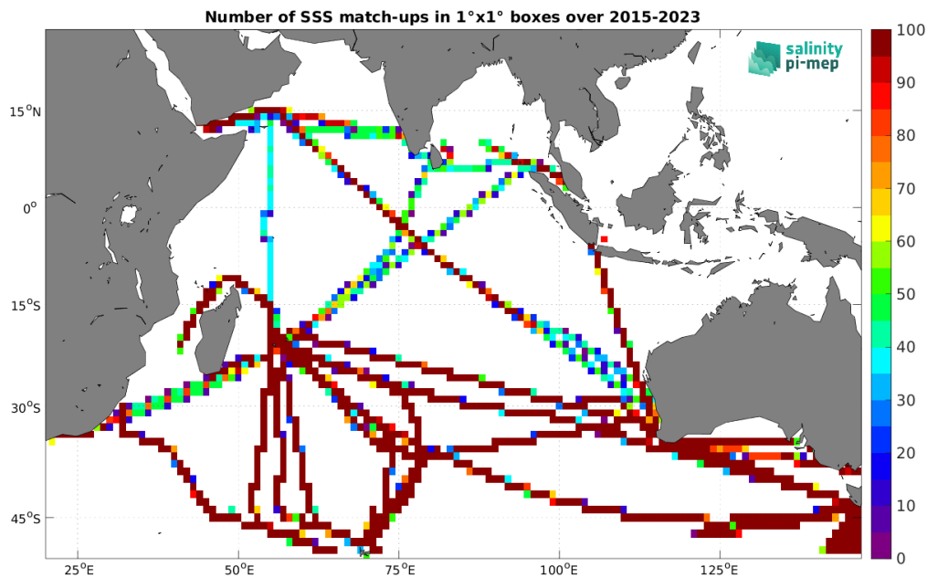
Figure 5: Number of SSS match-ups between TSG (LEGOS-DM) SSS and the SMAP SSS L3 v5.3 - Monthly (RSS) SSS product for the Indian Ocean Pi-MEP region over 1^\circ \times 1^\circ boxes and for the full satellite product period.
