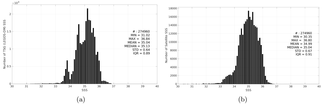
Figure 3: Histograms of SSS from TSG (LEGOS-DM) (a) and SMAP SSS L3 v5.3 - Monthly (RSS) (b) considering all match-up pairs per bins of 0.1 over the Indian Ocean Pi-MEP region and for the full satellite product period.
