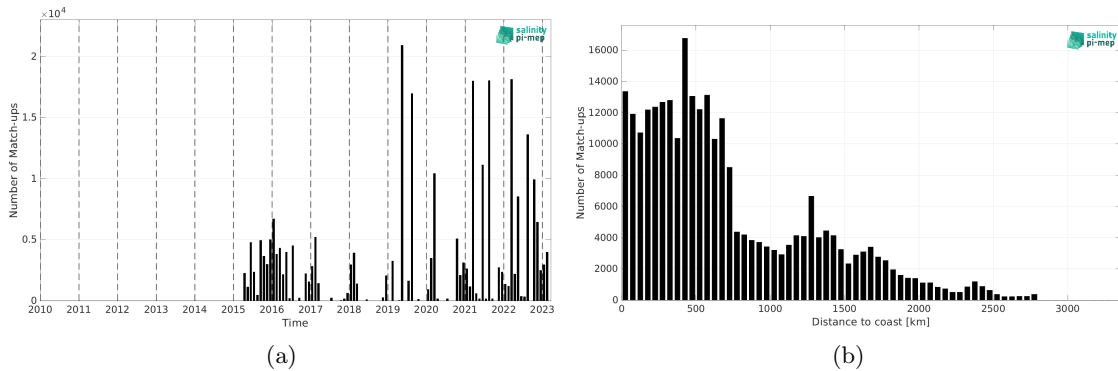
Figure 2: Number of match-ups between TSG (LEGOS-DM) and SMAP SSS L3 v5.3 - Monthly (RSS) SSS as a function of time (a) and as function of the distance to coast (b) over the Indian Ocean Pi-MEP region and for the full satellite product period.
