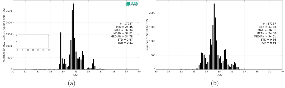
Figure 3: Histograms of SSS from TSG (GOSUD-Sailing-ship) (a) and SMAP SSS L3 v5.3 - Monthly (RSS) (b) considering all match-up pairs per bins of 0.1 over the Indian Ocean Pi-MEP region and for the full satellite product period.
