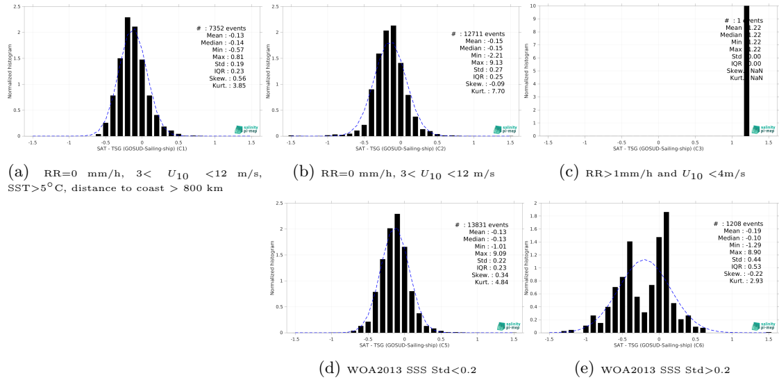
Figure 15: Normalized histogram of \Delta SSS (SMAP SSS L3 v5.3 - Monthly (RSS) - TSG (GOSUD-Sailing-ship)) for 5 different subdatasets corresponding to: RR=0 mm/h, 3 < U_{10} < 12 m/s, SST>5°C, distance to coast > 800 km (a), RR=0 mm/h, 3 < U_{10} < 12 m/s (b), RR>1mm/h and U_{10} < 4 m/s (c), WOA2013 SSS Std<0.2 (d), WOA2013 SSS Std>0.2 (e).
