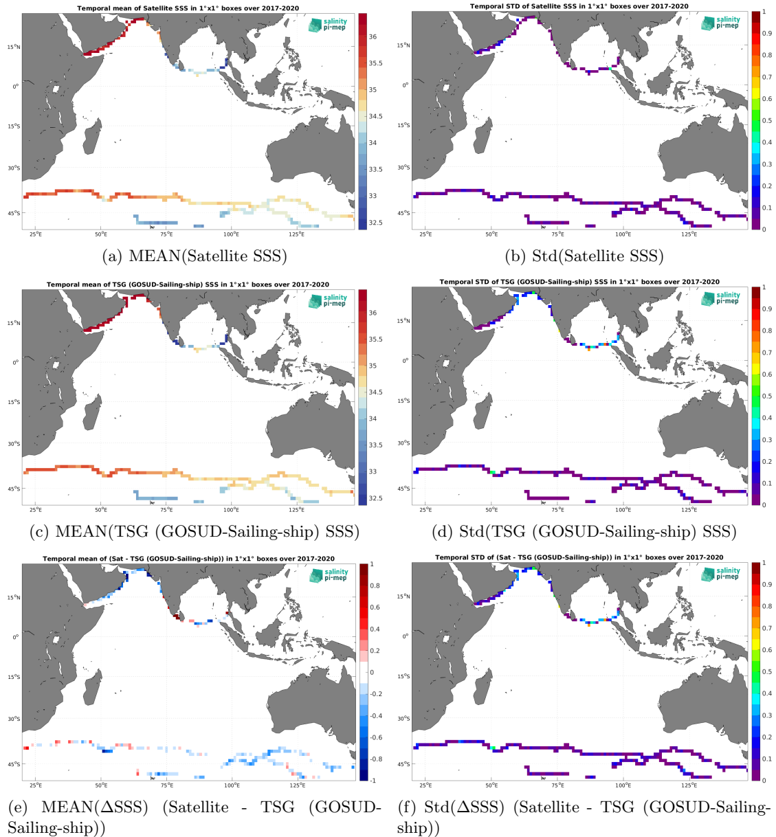
Figure 7: Temporal mean (left) and Std (right) of SSS from SMAP SSS L3 v5.3 - Monthly (RSS) (top), TSG (GOSUD-Sailing-ship) (middle), and of \Delta SSS (Satellite - TSG (GOSUD-Sailing-ship)). Only match-up pairs are used to generate these maps.
