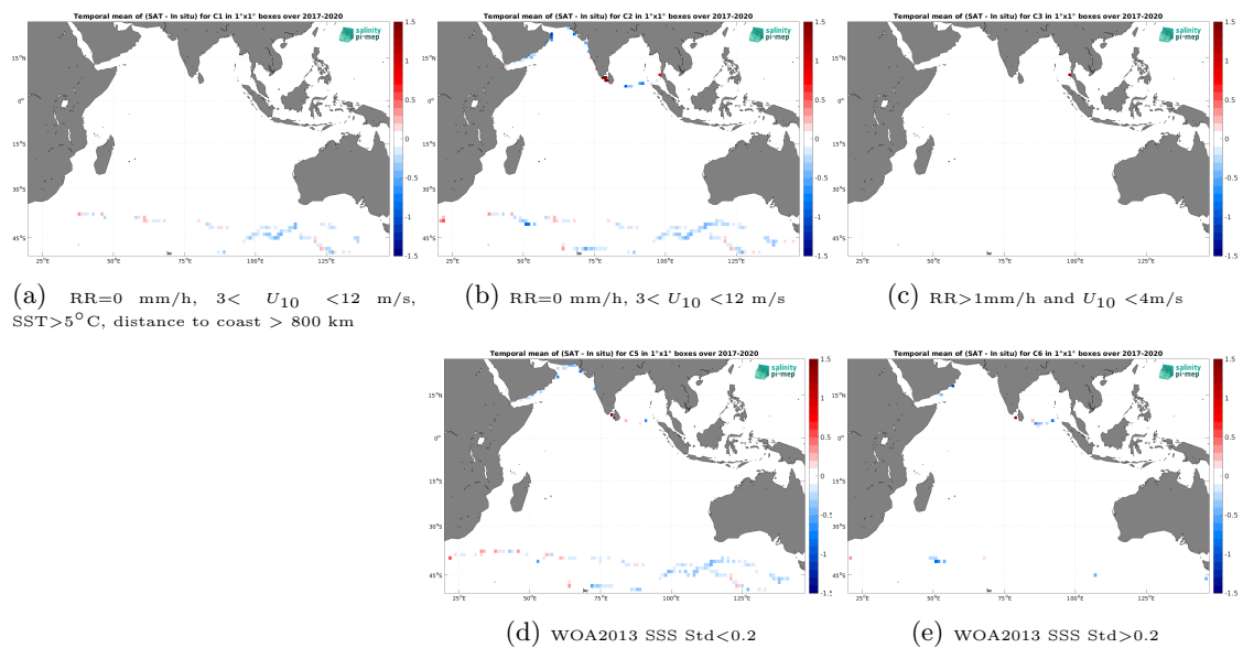
Figure 14: Temporal mean gridded over spatial boxes of size 1^\circ \times 1^\circ of \Delta SSS (SMAP SSS L3 v5.3 - Monthly (RSS) - TSG (GOSUD-Sailing-ship)) for 5 different subdatasets corresponding to: RR=0 mm/h, 3 < U_{10} < 12 m/s, SST > 5^\circ\text{C} , distance to coast > 800 km (a), RR=0 mm/h, 3 < U_{10} < 12 m/s (b), RR > 1\text{mm/h} and U_{10} < 4\text{m/s} (c), WOA2013 SSS Std < 0.2 (d), WOA2013 SSS Std > 0.2 (e).
