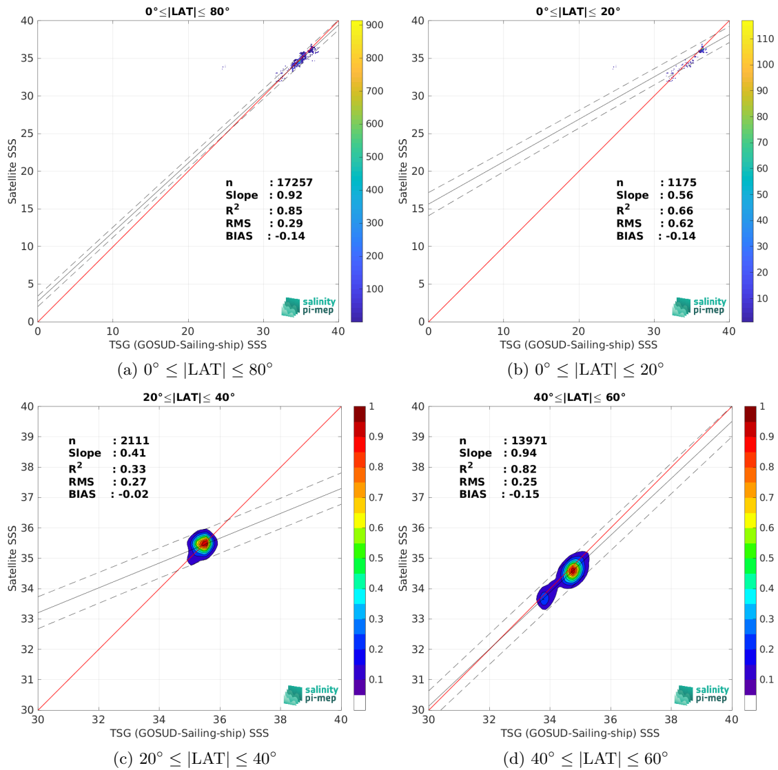
Figure 10: Contour maps of the concentration of SMAP SSS L3 v5.3 - Monthly (RSS) SSS (y-axis) versus TSG (GOSUD-Sailing-ship) SSS (x-axis) at match-up pairs for different latitude bands. For each plot, the red line shows x=y . The black thin and dashed lines indicate a linear fit through the data cloud and the \pm 95\% confidence levels, respectively. The number match-up pairs n , the slope and R^2 coefficient of the linear fit, the root mean square (RMS) and the mean bias between satellite and in situ data are indicated for each latitude band in each plots.
