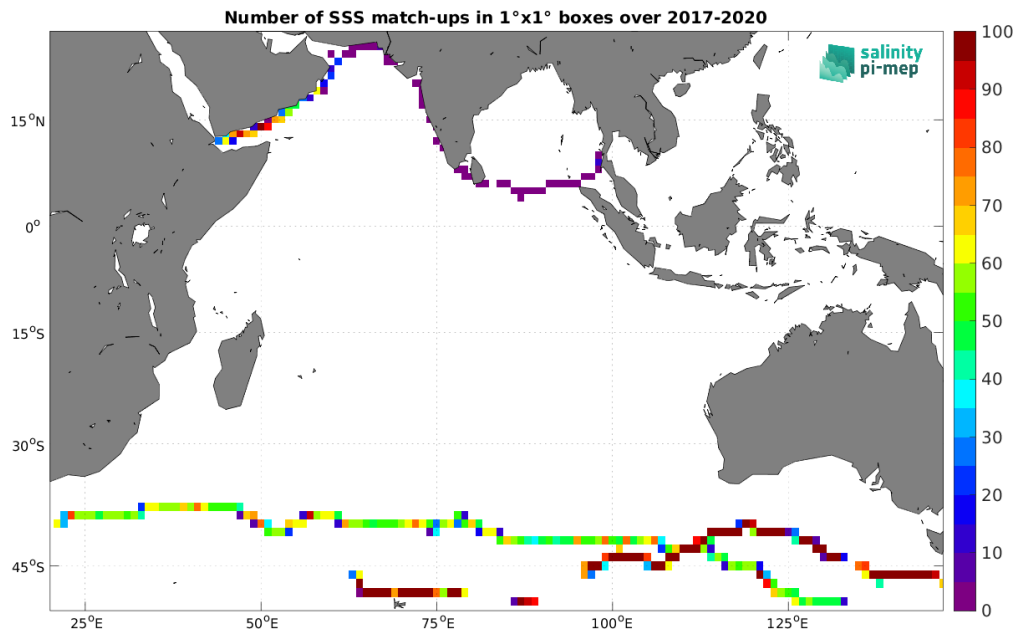
Figure 5: Number of SSS match-ups between TSG (GOSUD-Sailing-ship) SSS and the SMAP SSS L3 v5.3 - Monthly (RSS) SSS product for the Indian Ocean Pi-MEP region over 1^\circ \times 1^\circ boxes and for the full satellite product period.
