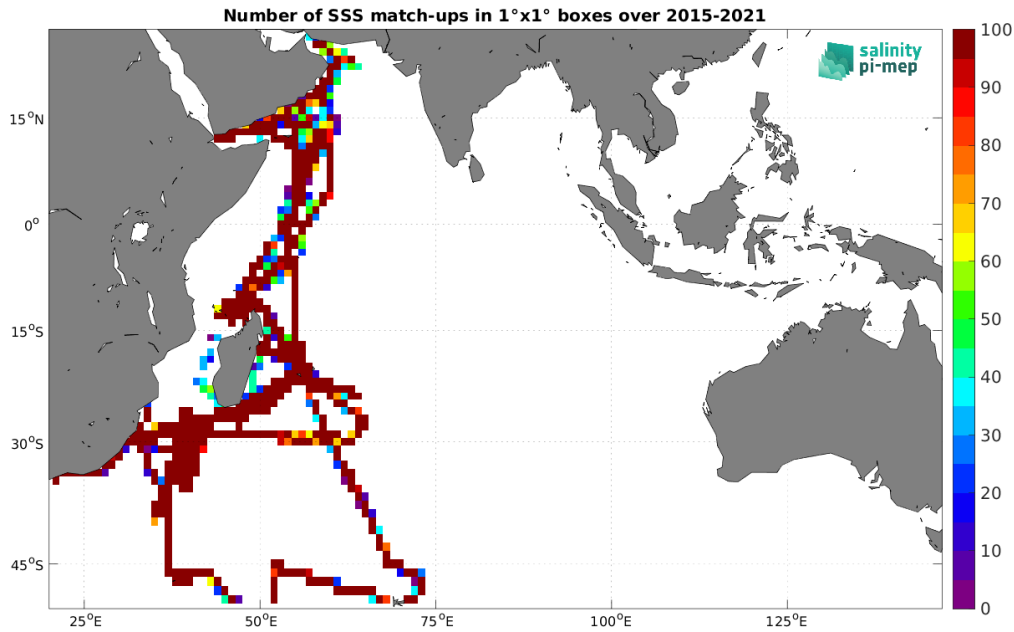
Figure 5: Number of SSS match-ups between TSG (GOSUD-Research-vessel) SSS and the SMAP SSS L3 v5.3 - Monthly (RSS) SSS product for the Indian Ocean Pi-MEP region over 1^\circ \times 1^\circ boxes and for the full satellite product period.
