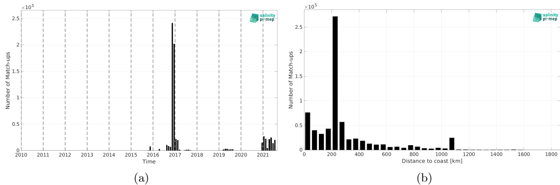
Figure 2: Number of match-ups between TSG (GOSUD-Research-vessel) and SMAP SSS L3 v5.3 - Monthly (RSS) SSS as a function of time (a) and as function of the distance to coast (b) over the Indian Ocean Pi-MEP region and for the full satellite product period.
