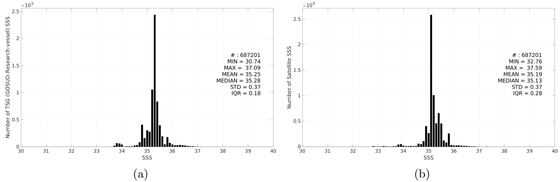
Figure 3: Histograms of SSS from TSG (GOSUD-Research-vessel) (a) and SMAP SSS L3 v5.3 - Monthly (RSS) (b) considering all match-up pairs per bins of 0.1 over the Indian Ocean Pi-MEP region and for the full satellite product period.
