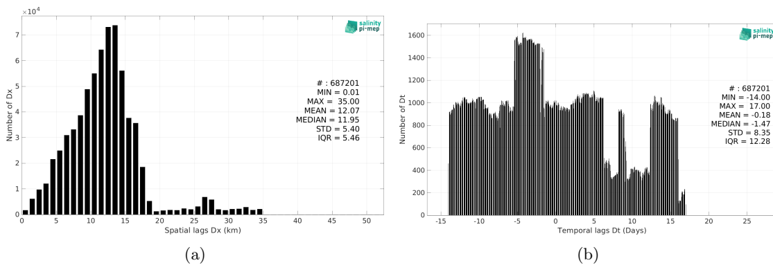
Figure 6: Histograms of the spatial (a) and temporal (b) lags between the location/time of the TSG (GOSUD-Research-vessel) measurement and the date of the corresponding SMAP SSS L3 v5.3 - Monthly (RSS) SSS pixel.
