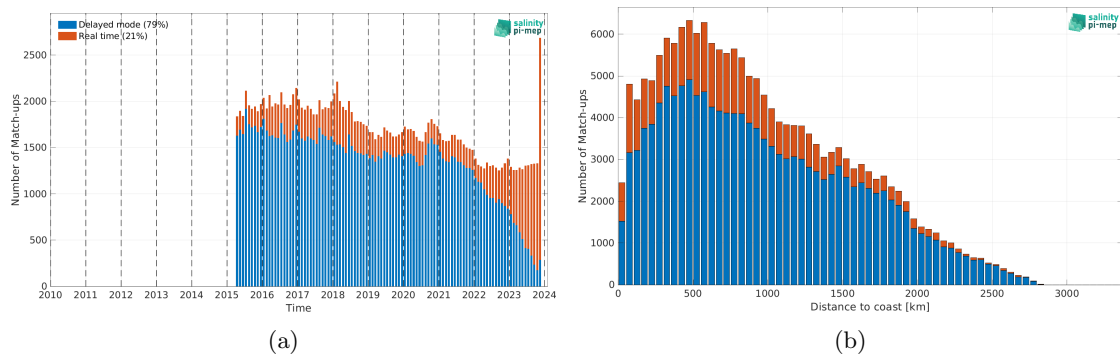
Figure 2: Number of match-ups between Argo and SMAP SSS L3 v5.3 - Monthly (RSS) SSS as a function of time (a) and as function of the distance to coast (b) over the Indian Ocean Pi-MEP region and for the full satellite product period.
