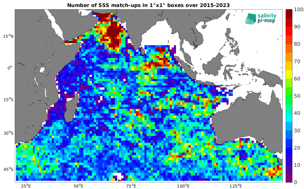
Figure 5: Number of SSS match-ups between Argo SSS and the SMAP SSS L3 v5.3 - Monthly (RSS) SSS product for the Indian Ocean Pi-MEP region over 1^\circ \times 1^\circ boxes and for the full satellite product period.
