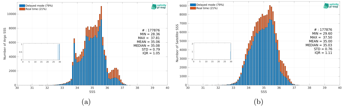
Figure 3: Histograms of SSS from Argo (a) and SMAP SSS L3 v5.3 - Monthly (RSS) (b) considering all match-up pairs per bins of 0.1 over the Indian Ocean Pi-MEP region and for the full satellite product period.
