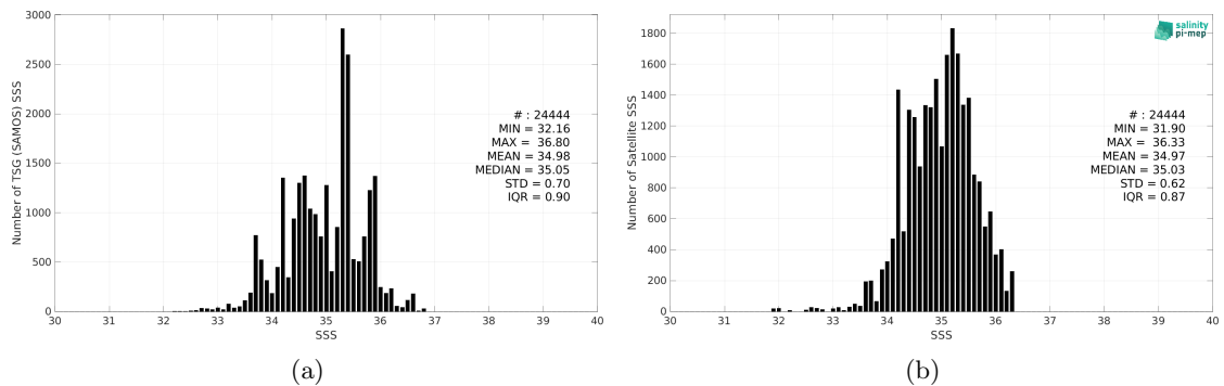
Figure 2: Histograms of SSS from TSG (SAMOS) (a) and SMAP SSS L3 v5 - 8-Day running (RSS) (b) considering all match-up pairs per bins of 0.1 over the Indian Ocean Pi-MEP region and for the full satellite product period.
