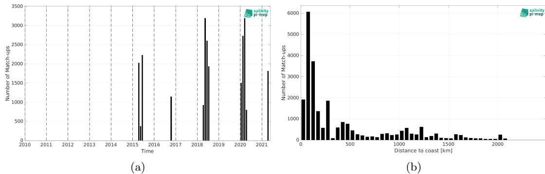
Figure 1: Number of match-ups between TSG (SAMOS) and SMAP SSS L3 v5 - 8-Day running (RSS) SSS as a function of time (a) and as function of the distance to coast (b) over the Indian Ocean Pi-MEP region and for the full satellite product period.
