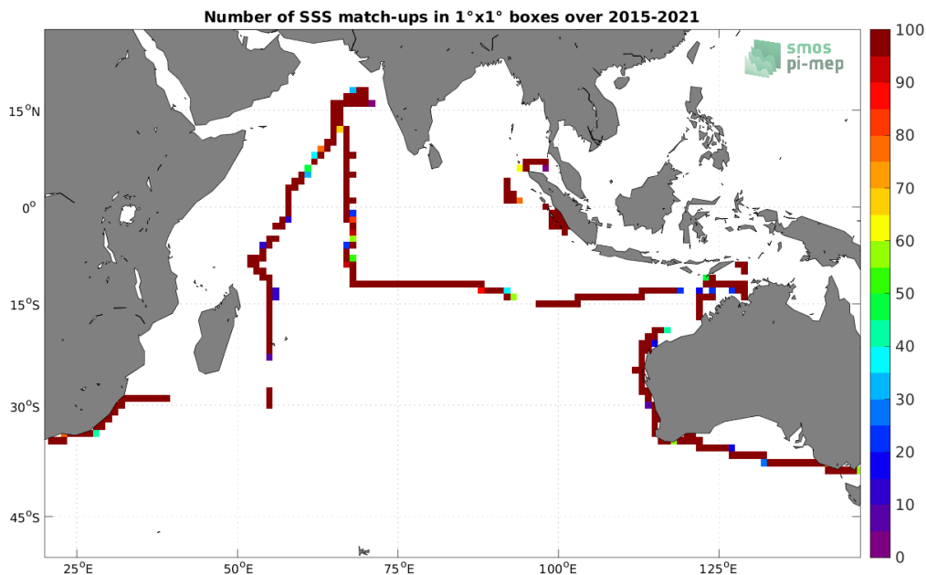
Figure 4: Number of SSS match-ups between TSG (SAMOS) SSS and the SMAP SSS L3 v5 - 8-Day running (RSS) SSS product for the Indian Ocean Pi-MEP region over 1^\circ \times 1^\circ boxes and for the full satellite product period.
