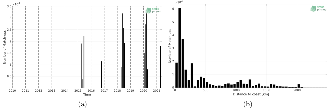
Figure 1: Number of match-ups between TSG (SAMOS) and SMAP SSS L3 v5 - 8-Day running (RSS) SSS as a function of time (a) and as function of the distance to coast (b) over the Indian Ocean Pi-MEP region and for the full satellite product period.
