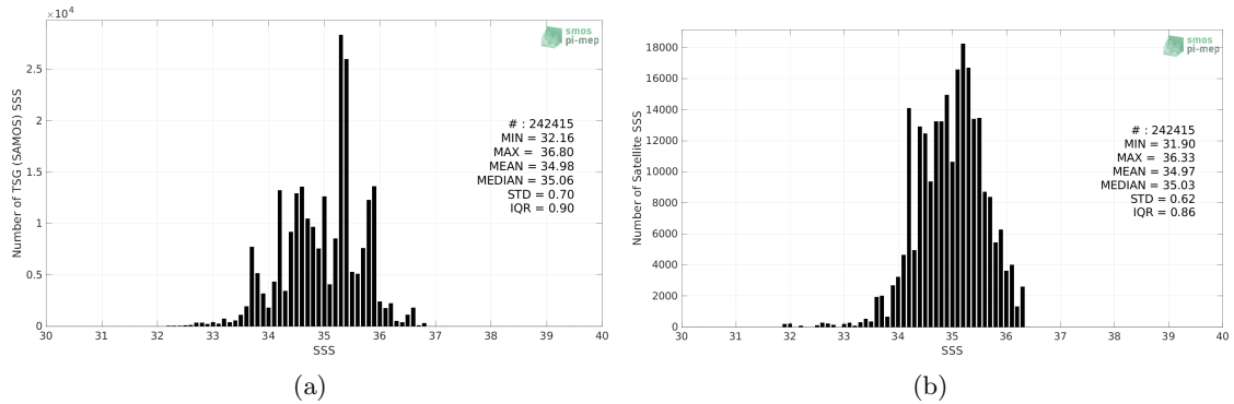
Figure 2: Histograms of SSS from TSG (SAMOS) (a) and SMAP SSS L3 v5 - 8-Day running (RSS) (b) considering all match-up pairs per bins of 0.1 over the Indian Ocean Pi-MEP region and for the full satellite product period.
