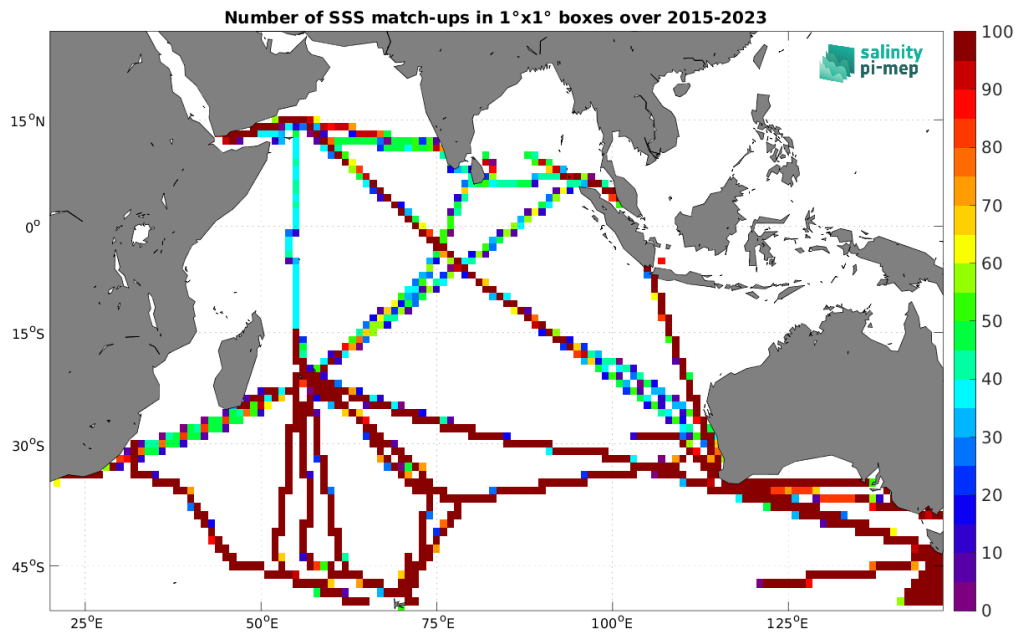
Figure 4: Number of SSS match-ups between TSG (LEGOS-DM) SSS and the SMAP SSS L3 v5 - 8-Day running (RSS) SSS product for the Indian Ocean Pi-MEP region over 1^\circ \times 1^\circ boxes and for the full satellite product period.
