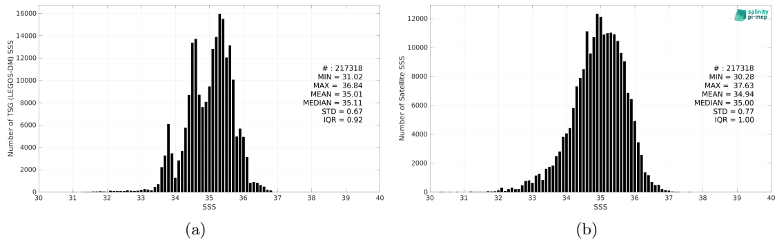
Figure 2: Histograms of SSS from TSG (LEGOS-DM) (a) and SMAP SSS L3 v5 - 8-Day running (RSS) (b) considering all match-up pairs per bins of 0.1 over the Indian Ocean Pi-MEP region and for the full satellite product period.
