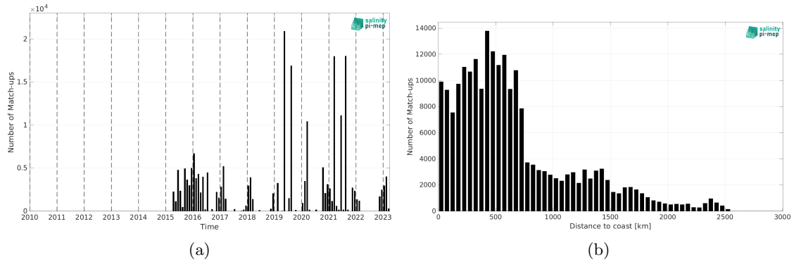
Figure 1: Number of match-ups between TSG (LEGOS-DM) and SMAP SSS L3 v5 - 8-Day running (RSS) SSS as a function of time (a) and as function of the distance to coast (b) over the Indian Ocean Pi-MEP region and for the full satellite product period.
